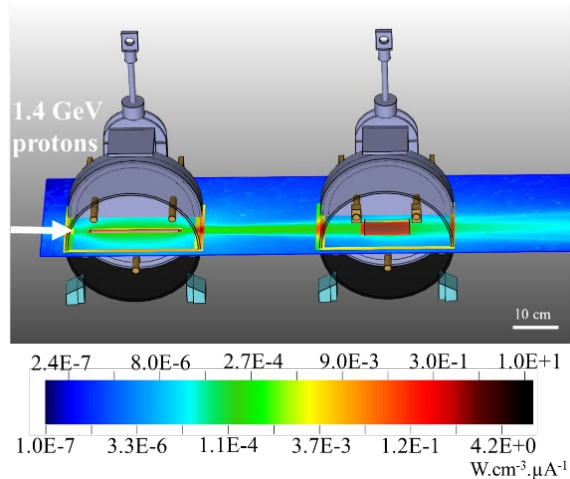
Figure 2: Visualisation of the ISOLDE (left) and MEDICIS target (right) irradiated by the 1.4 GeV proton beam. The deposited energy is represented in W.cm^{-3}.\mu A^{-1} .
