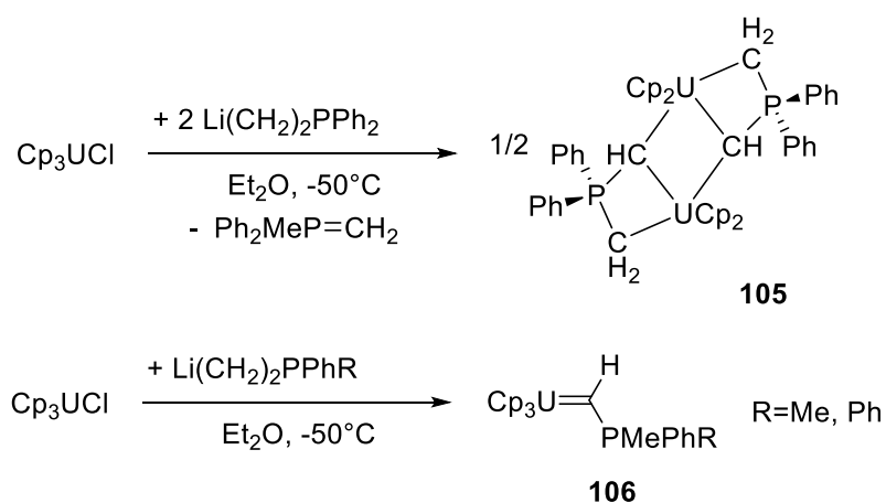
Scheme 104: Synthesis of uranium complexes of yldiide 73 following route A.
