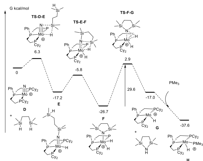
Scheme 5. Computed mechanism for the Si-H bond activations on the cationic \text{Mo}^{(\text{IV})} nitride complex. Gibbs free energies ( \text{kcal mol}^{-1} ) are given relative to "D + bisilane". Most H atoms have been omitted for clarity.
