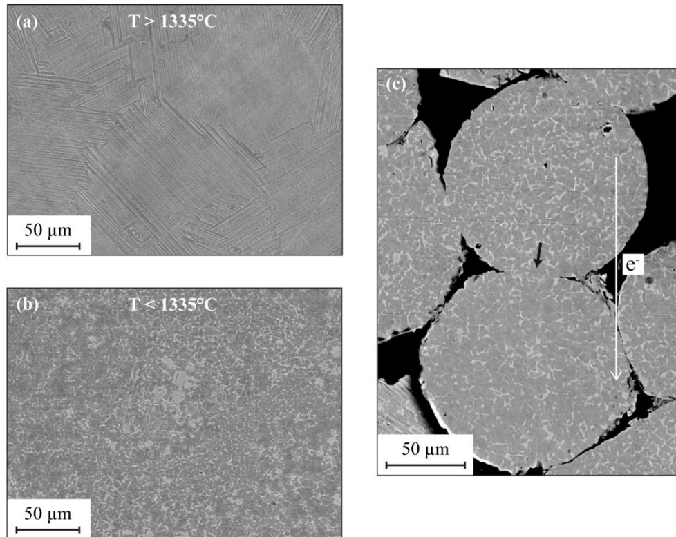
Fig. 4. Typical (a) Lamellar and (b) equiaxed microstructures of TiAl processed above and below 1335°C, respectively. (c) contact zone between two TiAl powder \approx 100\mu\text{m} particles in a sample processed by SPS at 926°C. The microstructure of the contact zone in the vicinity of the black arrow remains equiaxed, indicating no overheating above 1335°C. The white arrow indicates the average direction of the electron of the SPS current flowing through the sample.
