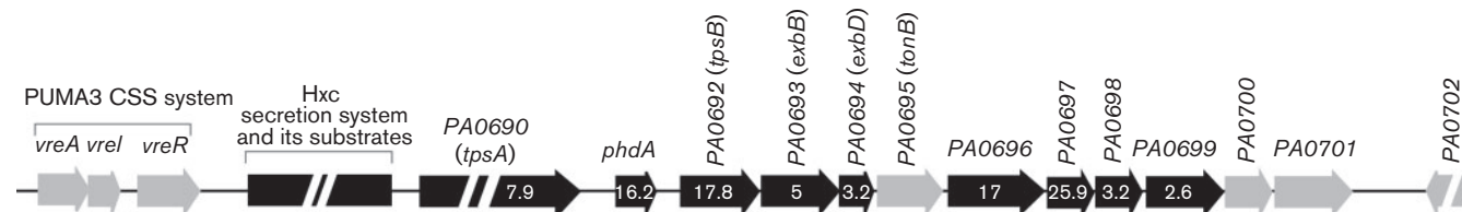
Fig. 1. Genetic organization of genes located downstream of the PUMA3 locus. Black arrows represent genes regulated by \sigma^{\text{Vrel}} (Llamas et al. , 2009) with their name or their respective PA number according to the PA01 genome annotation ( http://www.pseudomonas.com and Winsor et al. , 2011). Numbers inside the genes indicate the fold change obtained by microarray analysis (Llamas et al. , 2009). Grey arrows represent the neighbouring genes.
