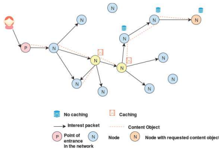
Fig. 2: Caching strategy.
