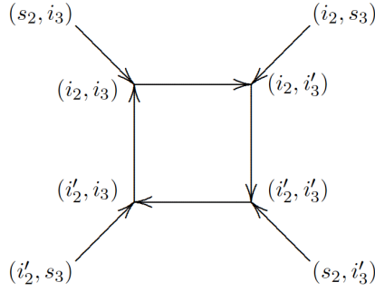
Figure 3: Diagram for the game in Example 3
