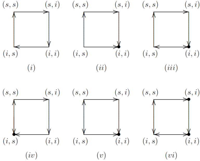
Figure 2: Diagrams for 2-by-2 Manipulator-Countermanipulator Games
