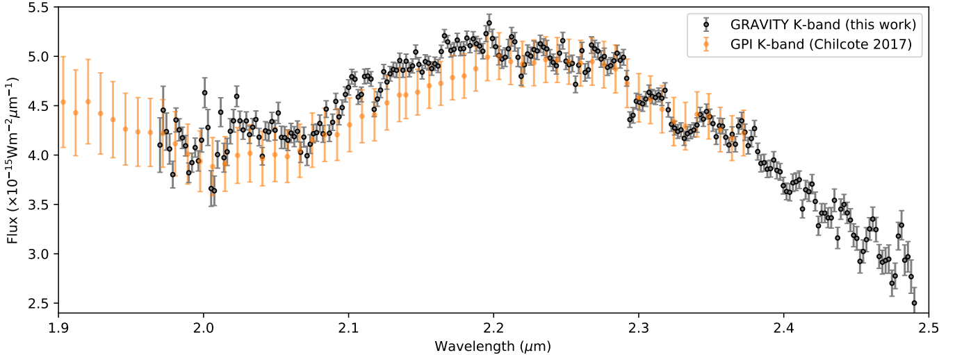
Fig. 1. Calibrated K -band spectrum of \beta Pictoris b, at R = 500 , extracted from the VLTI/GRAVITY observations (gray points). For comparison, the K -band part of the GPI spectrum from Chilcote et al. (2017) ( R \approx 70 ) is also overplotted (orange points). The error bars plotted for the GRAVITY spectrum only represent the diagonal part of the full covariance matrix.
