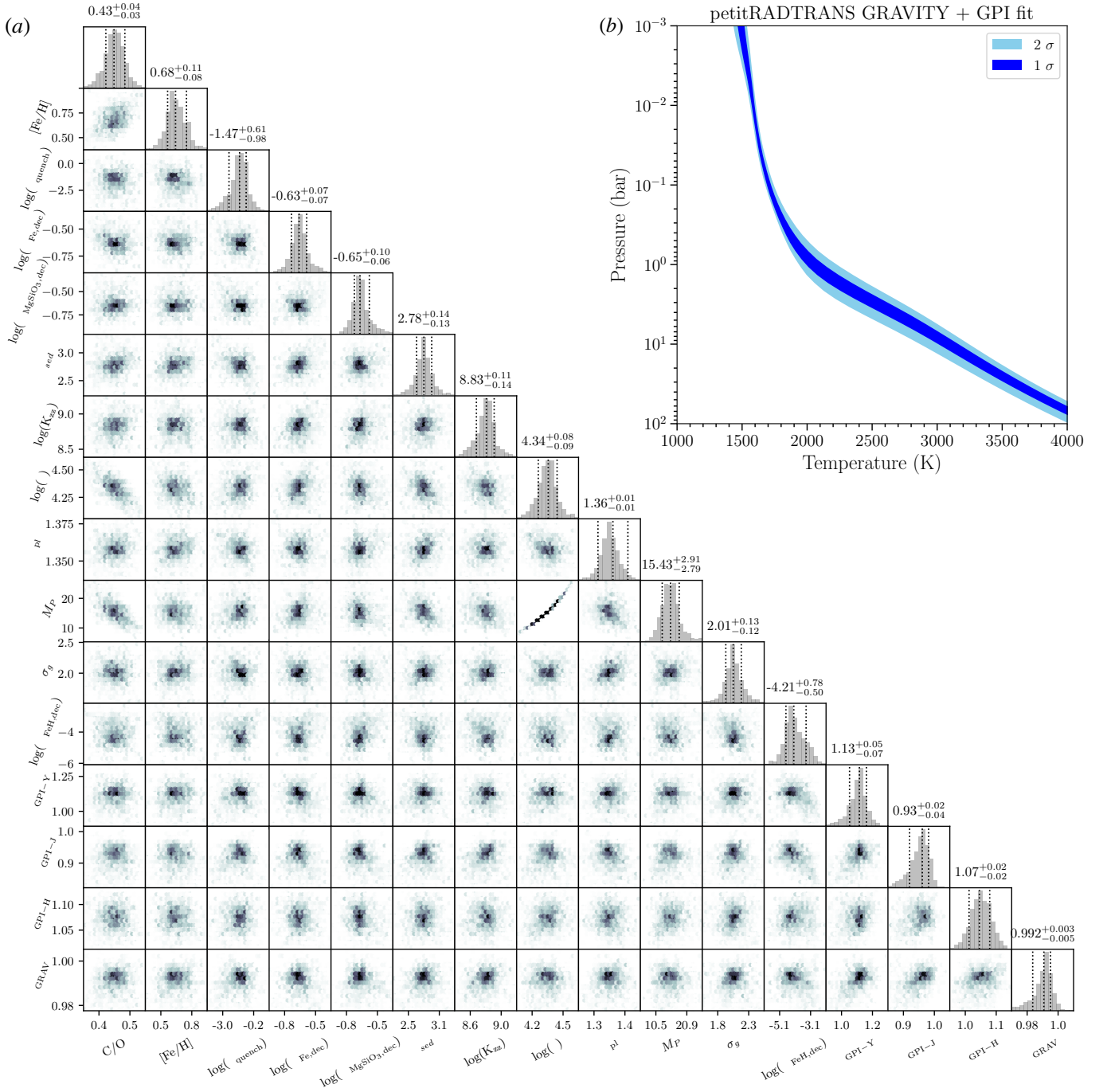
Fig. B.1. Panel a : projected 2-d posterior of the GRAVITY+GPI fit with petitRADTRANS (spectrum shown in Fig. 5), described in Sect. 4.3. See the text in Appendix B for a description of the parameters. Panel b : pressure-temperature envelopes obtained for the same retrieval. At every pressure, we plot the 16 to 84-percentile envelopes in dark blue, and the 2.5 to 97.5 percentile envelopes in light blue. If the temperature values were following a Gauss distribution, this would correspond to the 1 and 2 \sigma envelopes, respectively.
