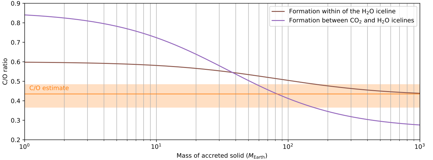
Fig. 7. Core-accretion scenario: evolution of the C/O ratio in the atmosphere of \beta Pic b as a function of the total mass of solid accreted by the protoplanet, for a formation between the H 2 O and the CO 2 icelines, or within the H 2 O iceline. The orange area gives the 68% confidence interval for the value of the C/O ratio.
