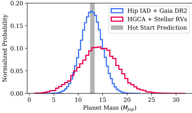
Fig. 3. Dynamical mass estimates of \beta Pic b using the two different methods described in Sect. 3.2. The shaded grey region is the 2\sigma uncertainty on the hot-start derived mass from Chilcote et al. (2017).
