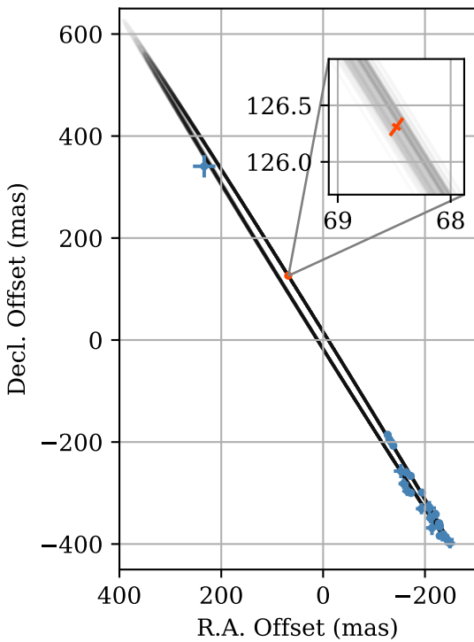
Fig. 2. Visual orbit of \beta Pic b. Plotted in black are possible orbits randomly drawn from the posterior using only relative astrometry (Sect. 3.1). Previous astrometric measurements used in the orbit fit are in blue. The GRAVITY measurement from this work is in red, with an inset plot that is zoomed in by a factor of \sim 2000 to display the uncertainties on this measurement.
