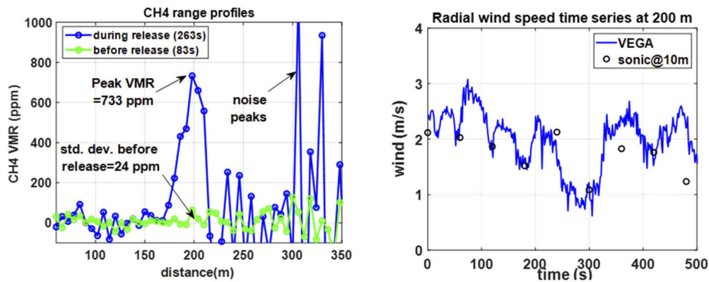
Fig. 7. Left: CH 4 volume mixing ratio range profiles measured at the VMR peak (263 s) and before the gas release (83 s). Right: Radial wind speed time series recorded just above the leak point by VEGA (at 200 m range), compared with a sonic anemometer located a few tens of meter away.
