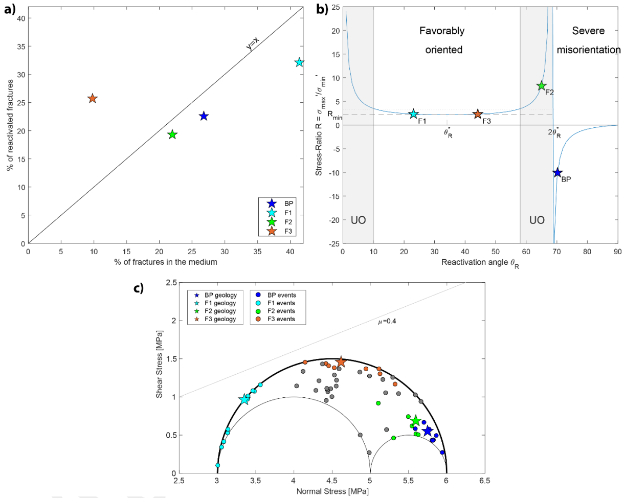
Figure 5 (a) Percentage of reactivated fractures in function of the percentage of fractures into the medium. (b) Stress ratio versus the reactivation angle \theta_R between \sigma_{max} axis and the fault plane for the four main fracture families (stars) that are reactivated. This figure is adapted from Sibson (1985), with \theta_R^* the optimal reactivation angle and the grey area showing the unfavorably fault orientation. In both panels, BP is dark blue, F1 is cyan, F2 is green and F3 is orange. (c) Stress state of the known geological structures (stars) and seismic events with a determined focal mechanism (dots) in a 3-D Mohr-Coulomb diagram. The grey line represents the rupture for a friction coefficient of 0.4 within the geomechanical stress state (Gugliemi et al. 2015) and the 3 half-circles the stress tensor.
