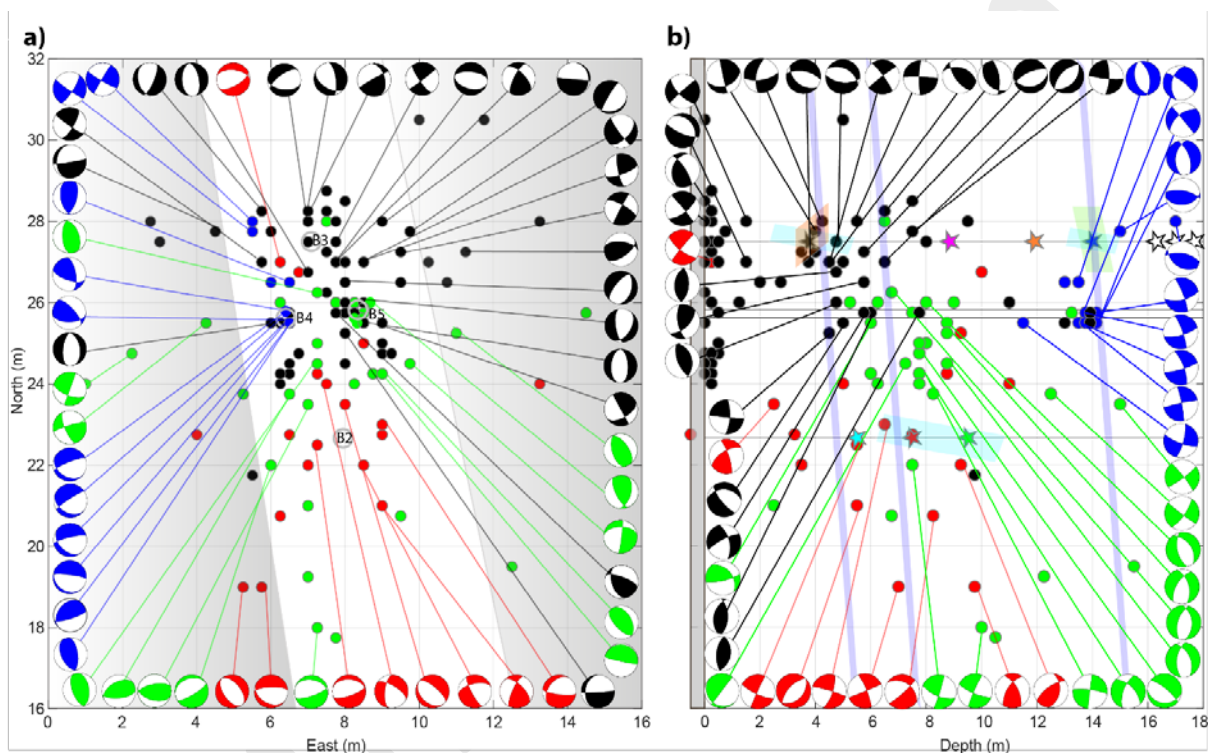
Figure 4 Focal mechanisms solution colored by test number (with Tests 2 in red, 3 in green, 9 in dark blue and 11 in black) in (a) a map view, and within the (b) depth-north direction. The figure (a) shows the focal mechanisms with a beach ball representation. Colored dots indicate the event locations. The white and grey areas show the gallery floor and walls. The grey circles show the borehole locations. The figure (b) presents the focal mechanisms into the Depth-North direction. The colored stars indicate the injection test locations. The grey plane shows the gallery floor. Finally, the main identified geological structures that intersect the injection intervals are shown as colored planes (blue for the BP, cyan for the F1, green for F2, and orange for F3).
