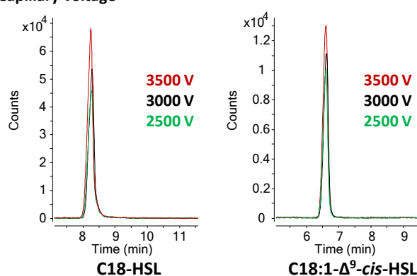
Fig. 5 Influence of the fragmentor voltage (a), the drying-gas temperature (b) and the capillary voltage (c) on the signal of C18-HSL and C18:1-Δ 9 -cis-HSL
