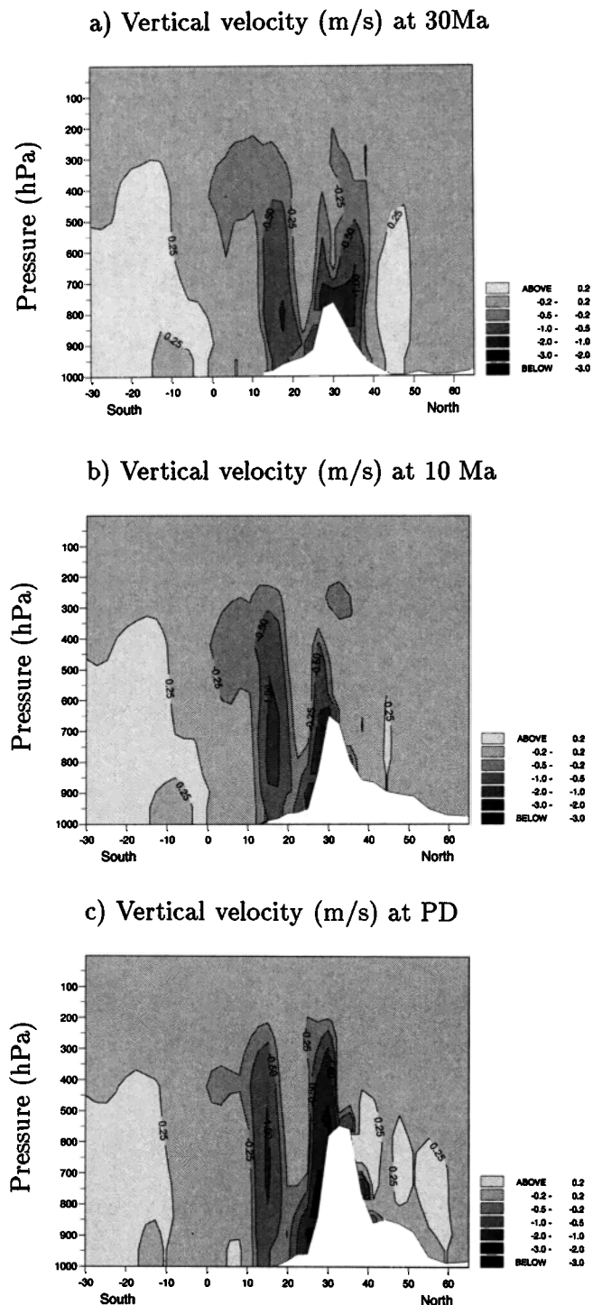
Figure 5. Mean vertical velocity in summer averaged in longitude between 80°E and 95°E at (a) 30 Ma (Exp2), (b) 10 Ma (Exp1), and (c) PD (Exp0). The vertical scale is pressure (hPa) and represents the atmosphere from sea level to 30 km height. Light gray areas are attributed to subsidence (positive values), dark gray indicates ascending motion (negative values), and white represents the orographic contour (Himalayas and Tibetan plateau).
