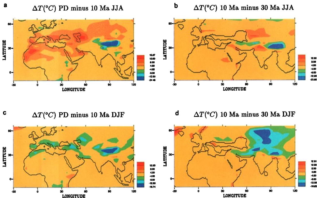
Plate 1. Mean temperature differences (°C) over Eurasia : (a) PD (Exp0) - 10 Ma (Exp1) in summer, (b) 10 Ma (Exp1) - 30 Ma (Exp2) in summer, (c) PD (Exp0) - 10 Ma (Exp1) in winter, and (d) 10 Ma (Exp1) - 30 Ma (Exp2) in winter. Cooling is in green and blue, warming is in orange and red, and no change is yellow.
