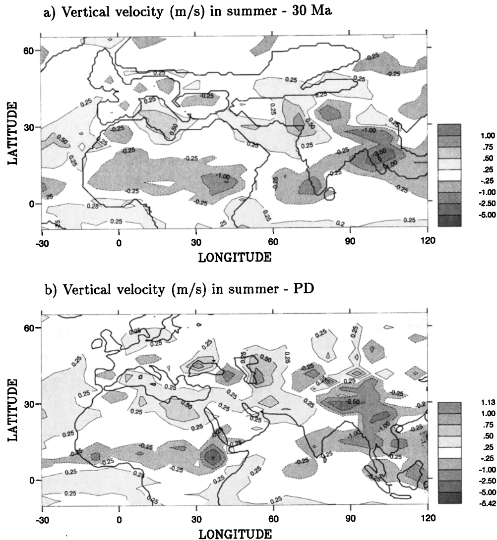
Figure 14. Mean vertical velocity (m/s) in summer at 500 hPa ( \approx 4500 m) at (a) 30 Ma (Exp2) and (b) PD (Exp0). Isolines are plotted for -5, -2.5, -1, -0.25, +0.25, +0.5, +0.75, and +1 m/s. Gray color represents vertical motion greater than \pm 0.25 m/s. Dotted line indicates ascending flow, and solid line shows subsidence.
