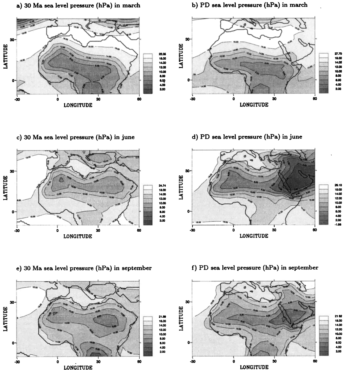
Figure 12. Sea level pressure (minus 1000 hPa) over Africa for the Oligocene (left) and PD (right). The gray areas represent the low-pressure cell, and white indicates pressure greater than 18 hPa (1018 hPa): (a) 30 Ma- Exp2 in March, (b) PD - Exp0 in March, (c) 30 Ma- Exp2 in June, (d) PD - Exp0 in June, (e) 30 Ma - Exp2 in September, and (f) PD - Exp0 in September.
