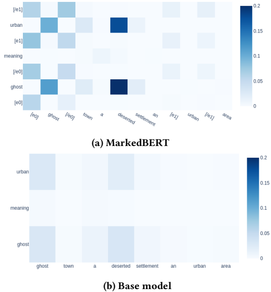
Figure 3: Attention map head between the query: “ghost meaning urban” and the passage: “ghost town a deserted settlement an urban area ...” tokens in the head 6 from layer 12 of MarkedBERT (a) and the Base model(b).
