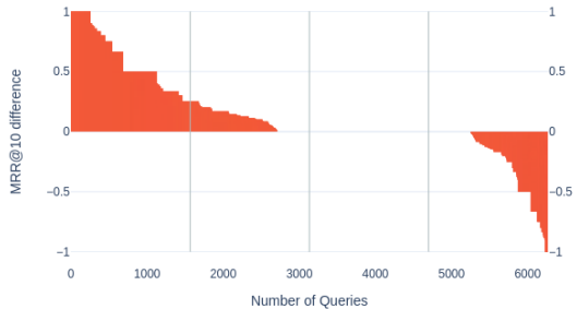
(a) MRR@10_{\text{MarkedBERT}} - MRR@10_{\text{Doc2query + BM25}}
