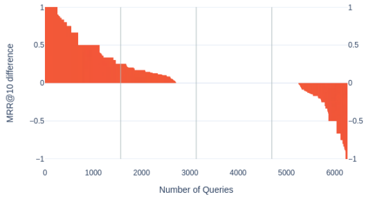
(a) MRR@10_{\text{MarkedBERT}} - MRR@10_{\text{Doc2query + BM25}}
