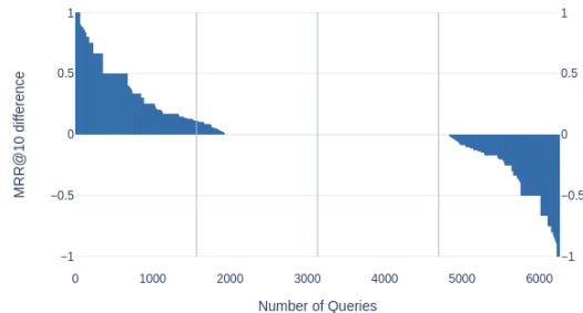
(b) MRR@10_{\text{MarkedBERT}} - MRR@10_{\text{Base}}
