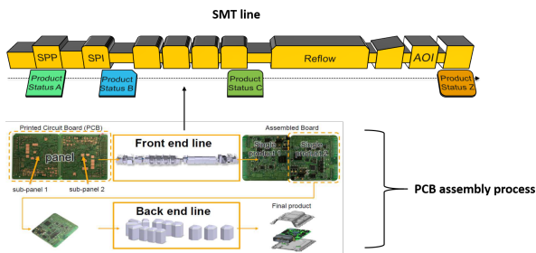
Figure 2: A schematic view of PCB assembly process
