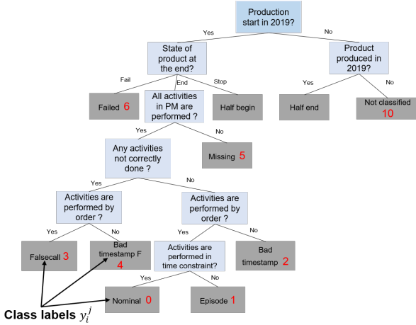
Figure 4: Decision Tree for product classification.
