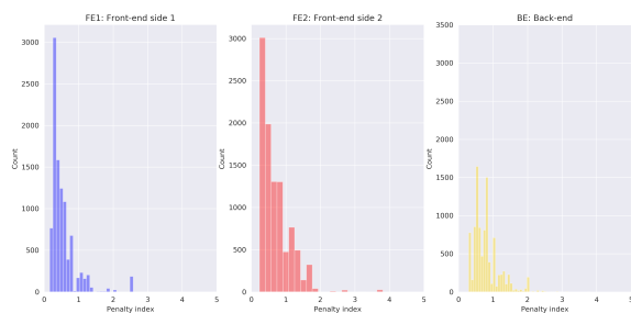
Figure 8: Product penalty indexes for each production phase
