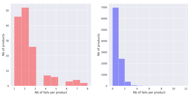
Figure 6: Distribution of Fail events per product. Left: Bad products, Right: Good products.
