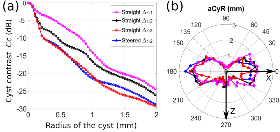
Figure 8. (a) Cyst contrast in dB, C_{c,dB} , computed for LSF of Thread 2 as a function of the radius of the cyst. The curves correspond to the different angular sampling periods and transmit modes; (b) polar representation of the anisotropic cystic resolution aCyR assessed on the LSF of Thread 2 for the different angular sampling periods and transmit modes.
