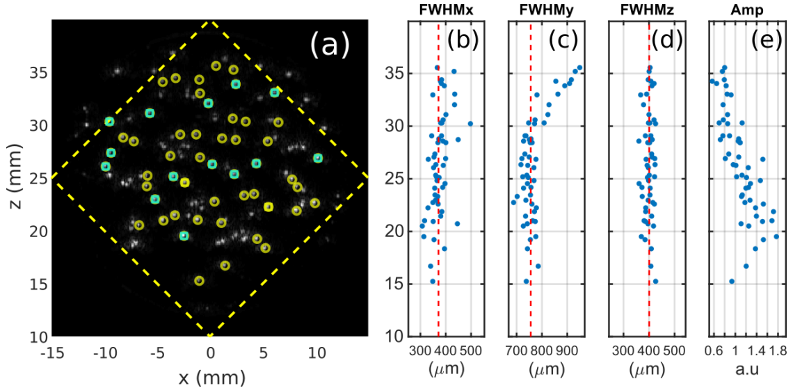
Figure 5. (a) MAP image along the y-axis of Ph1 for \Delta\alpha_2 in straight transmit. The 52 microspheres selected for the analysis are emphasized with yellow circular markers and the 16 microspheres kept for resolution estimations in translation-only mode are additionally emphasized with square cyan markers. (b)-(e): Resolution and amplitude of the 52 microspheres in the image are shown as a function of the z-coordinate. The red-dotted lines indicate the median values. For each FWHM graph, the range of abscissa is equal to 300\mu\text{m} .
