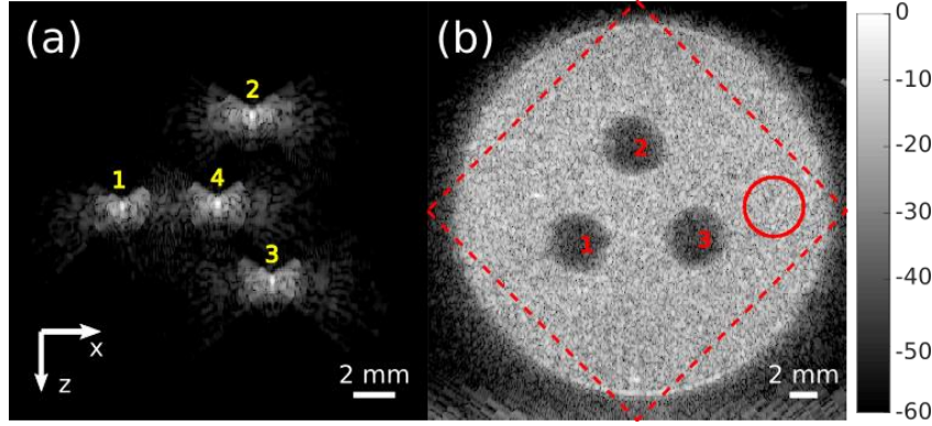
Figure 7. (a) xz -image of Ph3 (20 mm x 20 mm); (b) xz -image of Ph2 (30 mm x 30 mm). Both xz -images are at y = 0 and centered on x = 0 et z = 25 mm. They correspond to acquisitions performed in straight transmit at \Delta\alpha_2 with L = 30 mm. Numbers identify the threads (a) and holes (b), respectively. The speckle zone considered to calculate the image contrast is designated with a red circle in (b).
