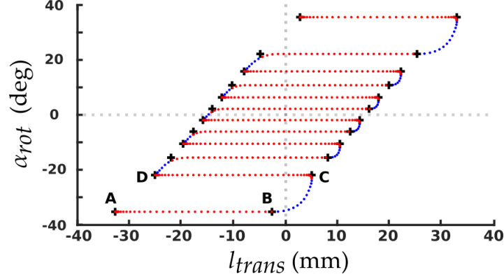
Figure 3. Successive motor positions for a rotate-translate scan with the angular sampling period \Delta\alpha_2 \approx 4^\circ . Positions used for reconstruction are shown with red markers. The black crosses represent targeted endpoints for the motor trajectories. The first four endpoints are notated A, B, C and D.
