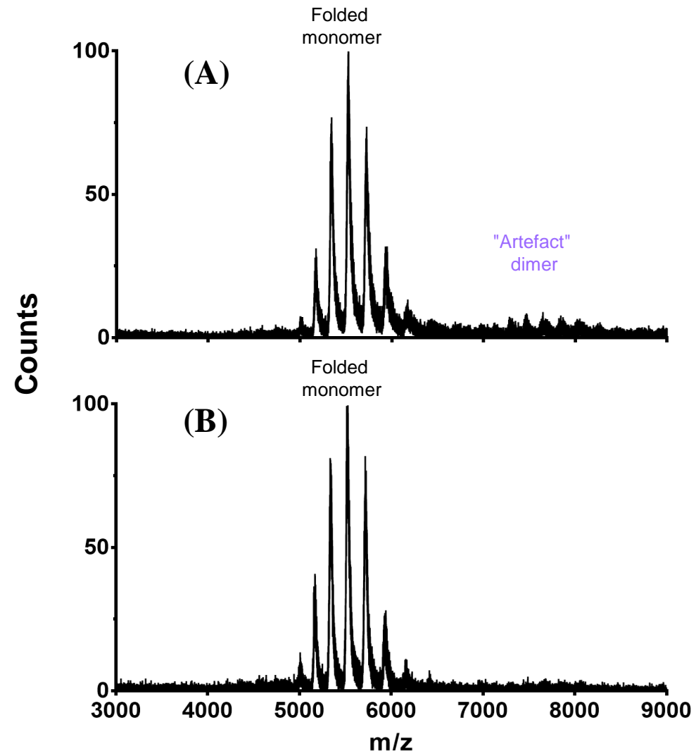
Figure 4: Mass spectra of monomeric Infiximab fraction at different in-source CID. (A), 25V, (B) 100 V. Mobile phase: ammonium acetate 150 mM, pH = 6.0 (10% IPA), other experimental conditions as mentioned in Figure 1.
