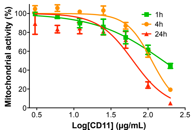
Fig S4. Effects of CD11 on the viability of A549 cells. Cells were treated with increasing concentrations (3-200 \mu\text{g/mL} ) of the CDs for 1, 4, and 24 h and viability was assessed with the MTT assay. Results are reported as % mitochondrial activity based on the control untreated cells normalized to 100 %. Data shown are representative of triplicate determinations (mean \pm SD).
