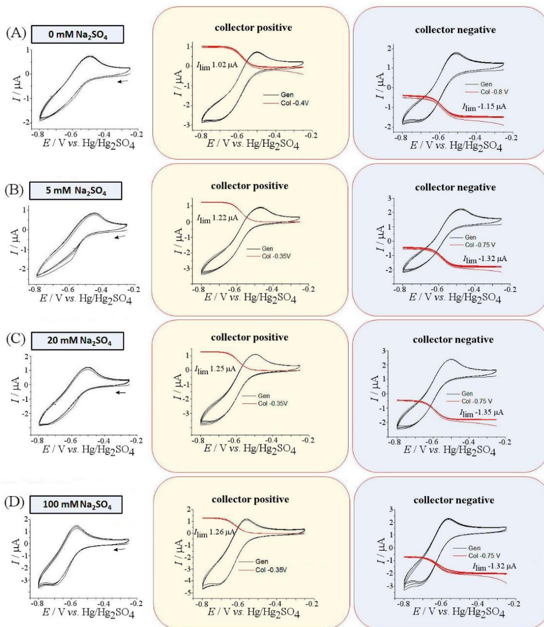
Figure 2. Cyclic voltammograms (scan rate 25 \text{ mV s}^{-1} ; four consecutive potential cycles) for a gold-gold dual-plate microtrench electrode immersed in 1 \text{ mM Ru}(\text{NH}_3)_6\text{Cl}_3 in aqueous (A) 0, (B) 5, (C) 20, and (D) 100 mM \text{Na}_2\text{SO}_4 . The generator electrode potential is scanning and the collector electrode potential is either floating (left column), set to the positive limit ( -0.35 \text{ V vs. Hg/Hg}_2\text{SO}_4 , middle column), or set to the negative limit ( -0.75 \text{ V vs. Hg/Hg}_2\text{SO}_4 , right column).
