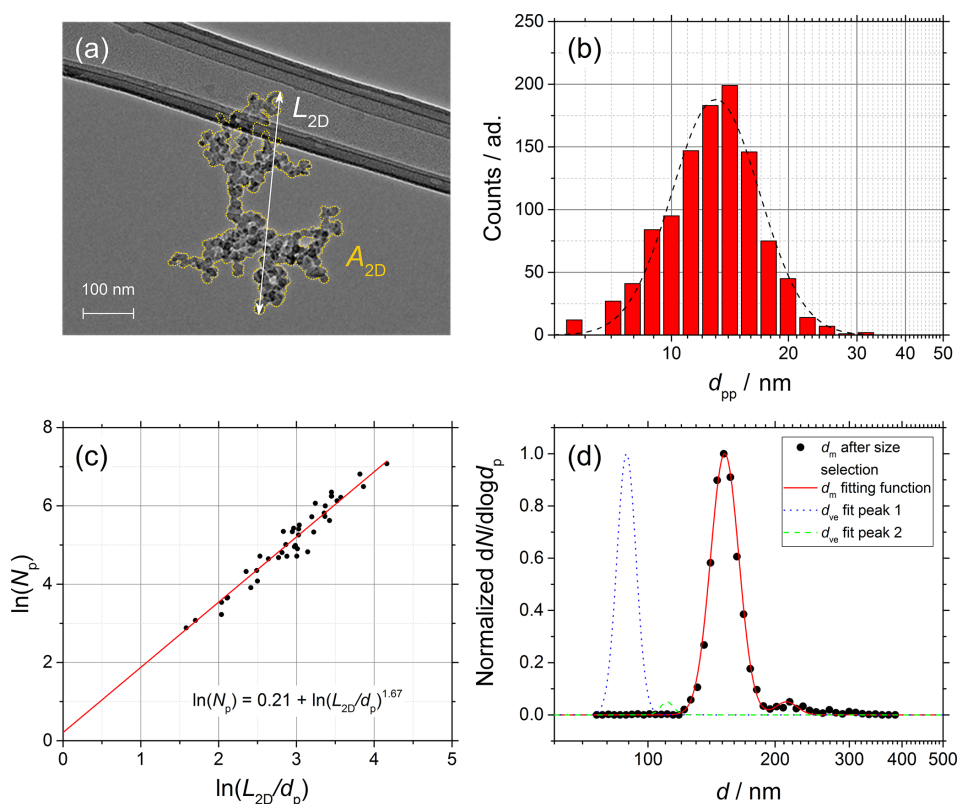
Figure 5. Soot sampled from the turbulent jet flame supplied with liquid kerosene at 70 mm HAB. (a) TEM picture of a soot aggregate showing L_{2D} and A_{2D} . (b) d_{pp} size distribution (red bars) and lognormal fit (dashed black line), d_{pp} = 13.0 nm (mass equivalent d_{pp} = 14.1 nm). (c) \ln(N_{pp}) vs. \ln(L_{2D}/d_{pp}) plot from which D_f is obtained (42 projections). (d) Normalized SMPS data and d_m fit after size selection at 150 nm (black data points and dashed red line) and morphology-corrected d_{ve} calculated using Eq. (11) showing a two-mode fit from Eq. (12) (dotted blue and dashed green lines).
