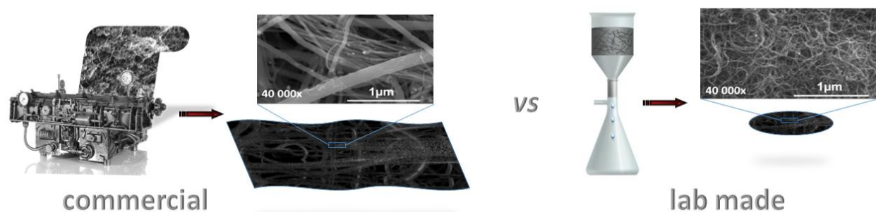
Figure 1.1: Illustration of fabrication procedures for commercial and lab-made buckypaper via mass production and lab-scale vacuum filtration, respectively.
