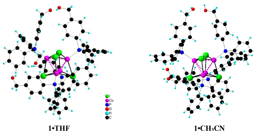
Figure 1. Molecular structure of [\text{Cu}_4\text{I}_4(\text{PPH}_2(\text{C}_6\text{H}_4\text{-CH}_2\text{OH})_4)] cluster in 1 •THF and 1 • \text{CH}_3\text{CN} . Structural disorder of the ligands is not shown for clarity. Cu-Cu contacts are represented in dashed pink lines.
