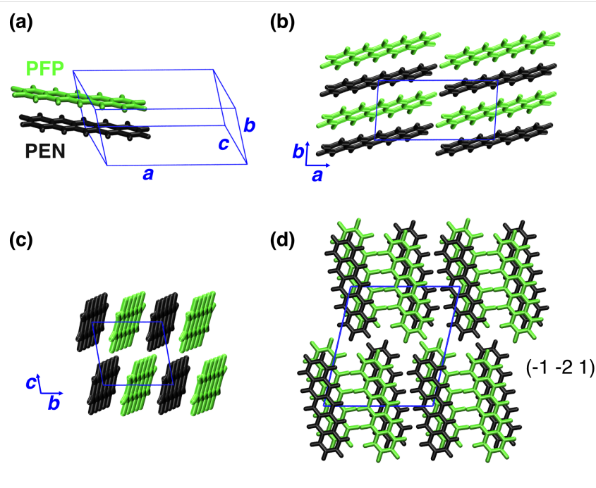
Figure 3: (a-c) Illustrations of the 1:1 crystal structure of PEN:PFP (black-green color) grown on HOPG. An almost identical unit cell was determined for the \text{SiO}_x substrate. (d) Top-view on the (-1 -2 1) plane, which was found as texture plane on HOPG (i.e., lies parallel to the HOPG (001) plane).
