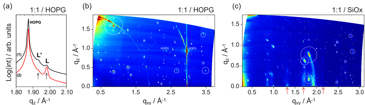
Figure 2: (a) XRD on nominally 300 Å thick films of 1:1 co-deposited PEN:PPF (curve 1) and of 75 alternating layers of PFP and PEN with a nominal thickness of 4 Å each (curve 2). Two diffraction features L and L' are observed close to the strong (002) reflection of HOPG; curves are vertically shifted for clarity. (b) GIXRD reciprocal space map of the film obtained by layered deposition (curve 2 in (a)). Reflections labeled with HOPG, the vertical feature at ca. q_{xy} = 3 \text{ \AA}^{-1} , and diffraction intensity on rings of constant q = \sqrt{q_z^2 + q_{xy}^2} stem from the HOPG substrate. (c) Reciprocal space map of a nominally 300 Å thick film of co-deposited PEN:PPF on SiO x ; red arrows indicate positions of weak vertical diffraction features along q_z which cannot be explained by the pure materials and are likely due to an additional upright-standing mixed phase of PEN:PPF. 28,32 In both figures, areas of the white circles correspond to calculated intensities for our structure solutions.
