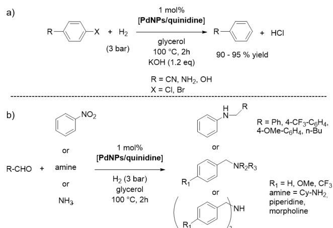
Scheme 2. PdNPs stabilized by quinidine applied in hydrodehalogenations (a) and in the synthesis of amines (b) [27].
