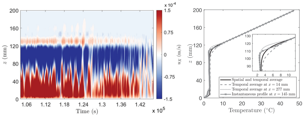
FIG. 17. Left: Horizontal average of the horizontal velocity u over a vertical cross section in the middle of the tank. The buffer layer can be seen above z = 120 mm. A stationary large-scale circulation is present in the convective layer, even if it appears quite perturbed at the end of the signal. Right: Temperature profiles along the z axis.
