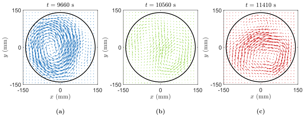
FIG. 10. Horizontal velocity vector fields in the stratified layer at different times. The laser sheet is located at z = 150 mm. The large-scale flow reverses from (a) to (c). Time between (a) and (c) is approximately half an hour. Maximum velocities are 0.1 mm/s.
