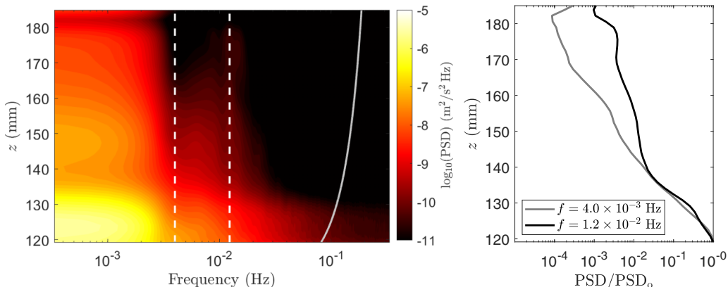
FIG. 9. Left: Power spectral density of the absolute velocity \sqrt{u^2 + w^2} above the convective layer. The grey curve shows the theoretical buoyancy frequency profile, assuming a linear profile for the temperature, from 4 °C to 35 °C. Right: Two selected profiles (taken at frequencies shown by dashed lines on the left graph) of the rescaled PSDs by the PSD at the top of the convective layer, i.e., z = 120 mm (denoted \text{PSD}_0 ). The PIV measurements are performed for 50 minutes and results (using the pwelch MATLAB function) are horizontally averaged at each height to obtain the averaged power spectral density.
