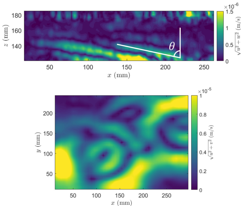
FIG. 8. Velocity fields showing IGWs propagating. Top: Velocities in (x, z) plane. The signal is frequency filtered to enhance the visualization of oscillatory motions: only frequencies between 0.02 and 0.03 Hz are shown, propagating at an angle of roughly 75^\circ with the vertical. The angle of propagation is the angle between the constant phase line and the vertical. Bottom: Velocities in (x, y) plane located at z \approx 125 mm. In the (x, y) plane, IGWs take the form of oscillating rings. Note that this figure is from a previous experiment without any internal cylinder and is therefore only displayed here as an illustration of the IGWs seen from above.
