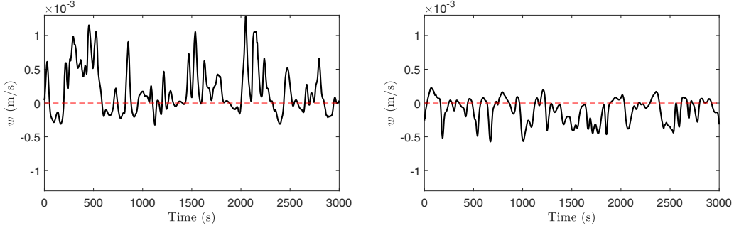
FIG. 3. Time evolution of the vertical velocity w within (left) upward plumes at x = 200 mm, z = 45 mm and (right) downward structures at x = 100 mm, z = 95 mm.
