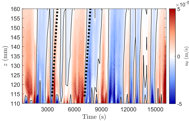
FIG. 12. Reversals of the large-scale flow. z = 115\text{--}120 mm is the convective/buffer layer interface. Ascending plumes often perturb the buffer layer flow. The velocity was measured at 11 heights, marked by each tick in the vertical axis of the figure, and interpolated in between. The slope of the black dot lines represents the viscous coupling phase velocity.
