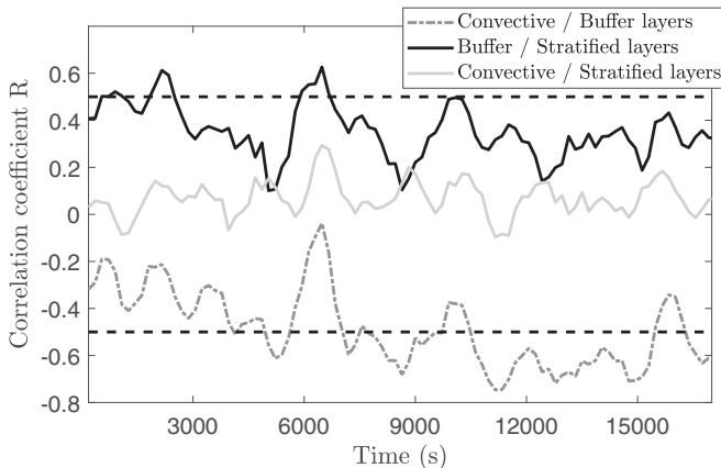
FIG. 15. Velocity correlation between the three layers. Dashed black lines are the -0.5 and 0.5 values. Correlation coefficient are window averaged over 10 min to smooth the curve.
