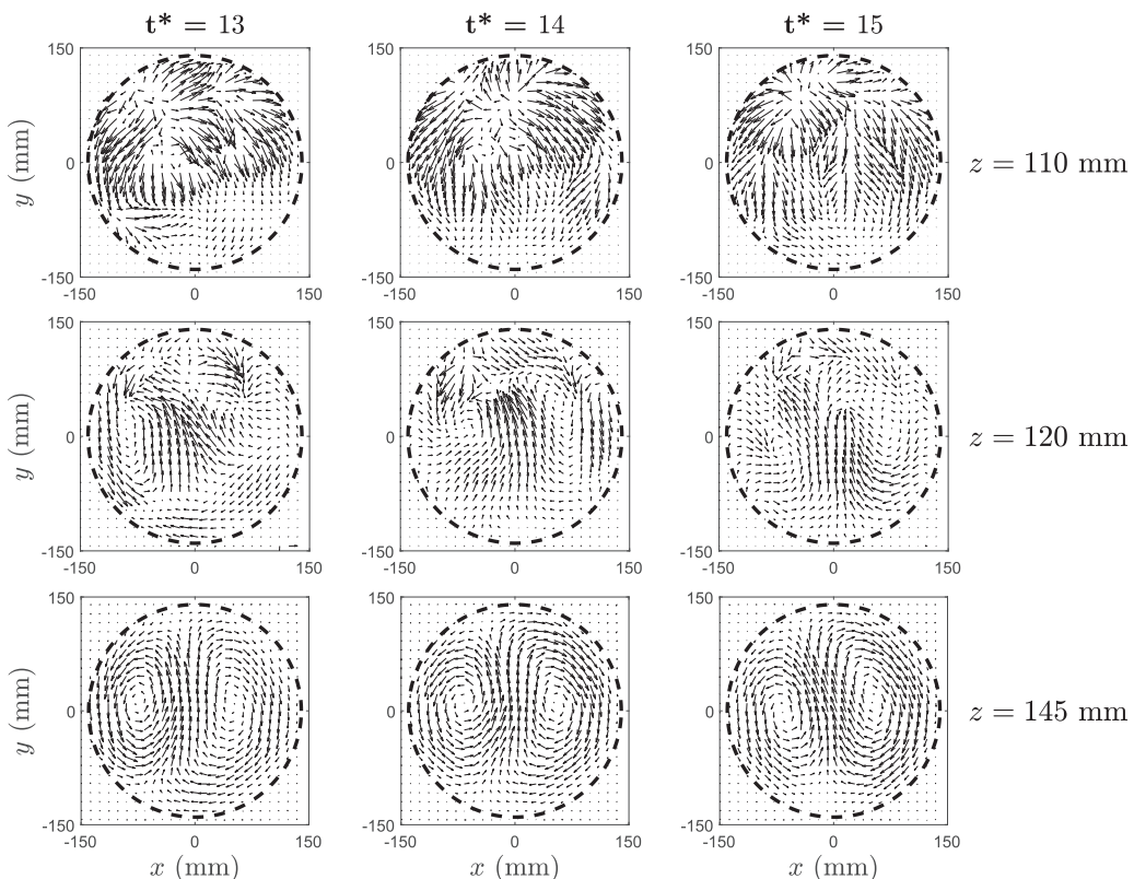
FIG. 13. Velocity vector fields in the horizontal plane. Different columns represent different sweeping cycles t^* (one sweeping cycle corresponds to the 11 steps needed to go from the lowest position z = 110 mm to the highest position z = 160 mm). Different rows represent different heights within the same sweeping cycle: the first row is the top of the convection z = 110 mm, the second row is in the buffer layer z = 120 mm, and the third row is in the stratified layer z = 145 mm. Convective plumes are easily noticeable on the first row fields.
