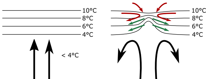
FIG. 7. Sketch of the thermal coupling between the convective and buffer layers. On the left, a cold plume moves upwards towards the interface between the two layers. On the right, isotherms are deflected due to the impact.
