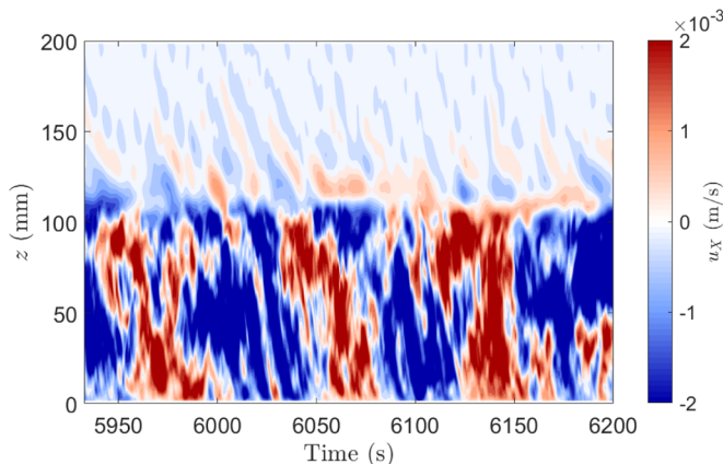
FIG. 22. Horizontal average of the horizontal velocity u over a vertical cross section in the middle of the numerical domain for \text{Pr} = 0.1 .
