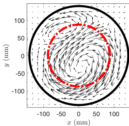
FIG. 11. Criterion used to extract a significant value for the large-scale flow and its direction: the azimuthal velocity is averaged over the ring shown in red.
