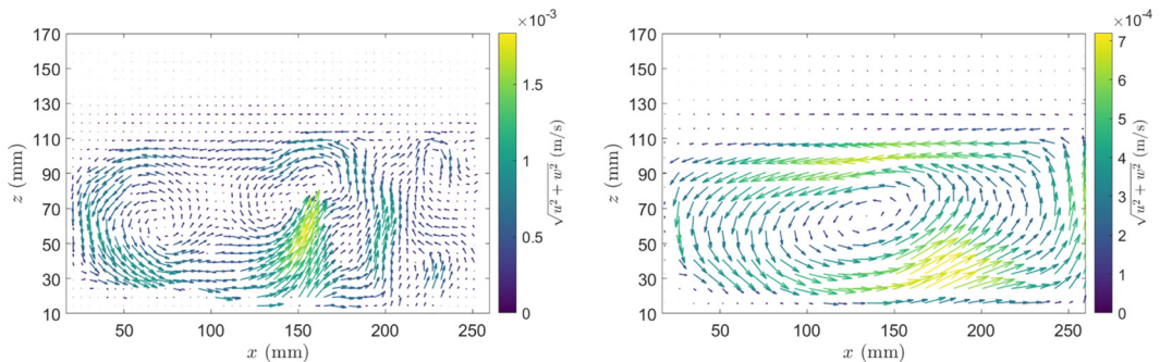
FIG. 2. Left: Instantaneous velocity field. An ascending plume is visible at x = 150 mm, and transported by the large-scale circulation. Right: Large-scale circulation in the convective layer obtained by time-averaging velocities over a 50 minute signal. The large-scale circulation is a counterclockwise cell. No inversion of the circulation has been seen in our experiment. The velocities under z = 10 mm are noisy and thus not shown here. Maximum instantaneous velocities are 2.5 times bigger than the maximum averaged velocities. The left edge of the cylinder is located at x = 19 mm and the center of the cylinder is at x = 160 mm. Approximately 40 mm of the right side of the cylinder is not captured with our PIV measurements.
