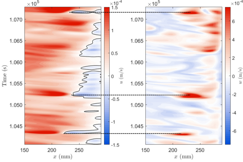
FIG. 19. Left: Spatio-temporal diagram of the horizontal velocity u at z = 128 mm. Right: Spatio-temporal diagram of the vertical velocity w at z = 108 mm. The event at t \approx 1.052 \times 10^5 s is shown in Fig. 18.
