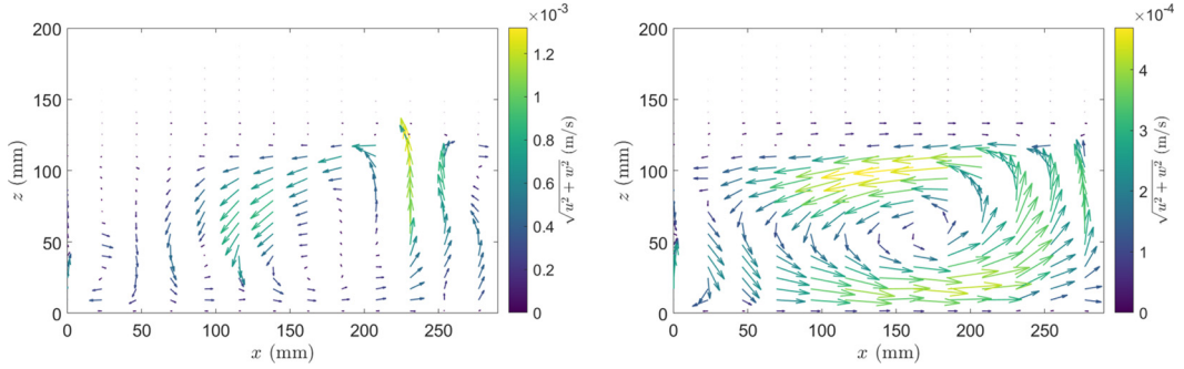
FIG. 16. Left: Instantaneous velocity field. An ascending plume is visible at x = 230 mm. Right: Large-scale circulation in the convective layer obtained by time averaging velocities over a 50 minute recording. The large-scale circulation is a counterclockwise cell. Maximum instantaneous velocities are 3 times bigger than the maximum averaged velocities.
