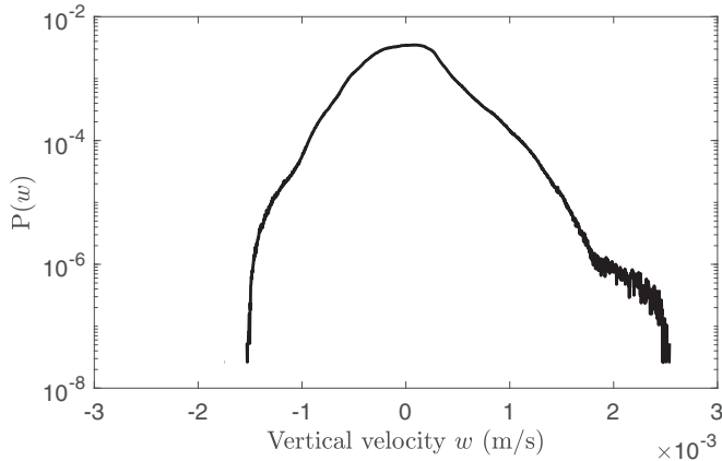
FIG. 5. Probability density function of the vertical velocities in the convective layer. All PIV points under z = 110 mm have been used to compute the PDF.
