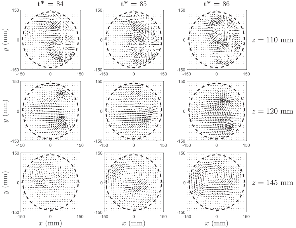
FIG. 14. Same as Fig. 13 but for different sweeping cycles. Note that in this set of velocity fields the buffer and stratified layers are less correlated than they are in Fig. 13.
