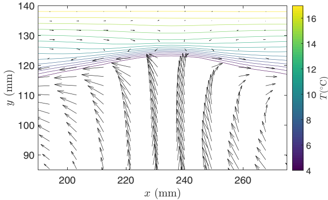
FIG. 18. Velocity field and temperature isotherms at the end of an upward plume impact on the interface.
