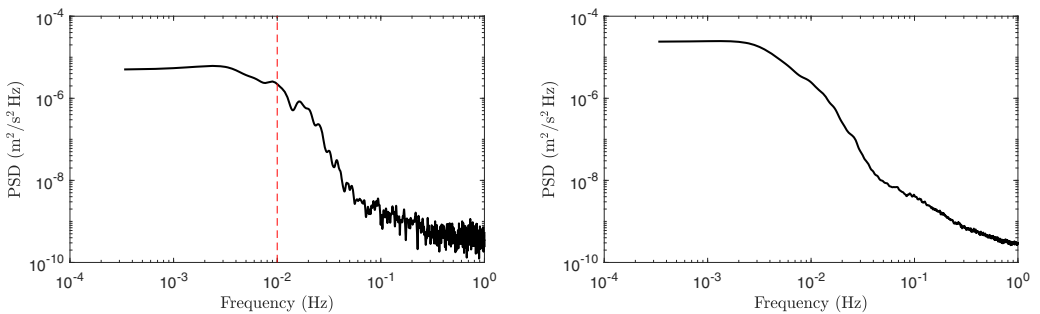
FIG. 4. PSD for the vertical velocity fluctuations. Left: PSD computed at a single point x = 100 mm, z = 95 mm (signal shown in Fig. 3 right). The plume forcing frequency can be seen around f = 10^{-2} Hz (red dashed line). Right: PSD spatially averaged over the whole convective cell in the measured (x, z) plane (all points above z = 10 mm and below z = 110 mm).
