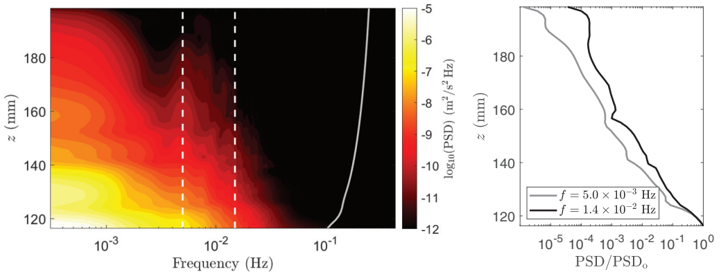
FIG. 20. Left: Power spectral density of the absolute velocity \sqrt{u^2 + w^2} in the buffer and stratified layers. The grey curve shows the buoyancy frequency profile computed from the spatial and temporal average of the temperature field. Right: Two selected profiles (taken at frequencies shown by dashed lines on the left graph) of the rescaled PSDs by the PSD at the top of the convective layer, i.e., z = 118 mm.
