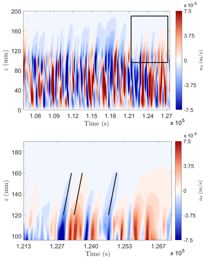
FIG. 21. Spatio-temporal diagrams of the azimuthal averaging of the azimuthal velocity inside a virtual cylinder of radius r = 140 mm. The bottom figure is a zoom on the stratified zone, delimited in the top figure by the black square. The slope of the black lines shows the theoretical viscous diffusive time.
