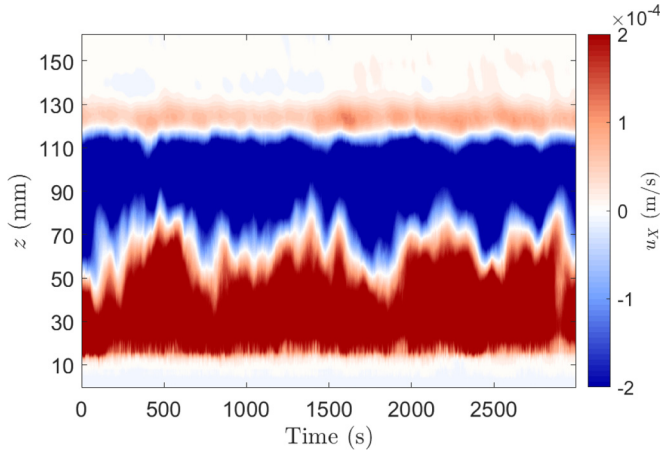
FIG. 6. Time evolution of the horizontal average of the horizontal velocity, noted u_x . Red (resp. blue) regions correspond to mean flow going towards the right (resp. left).
