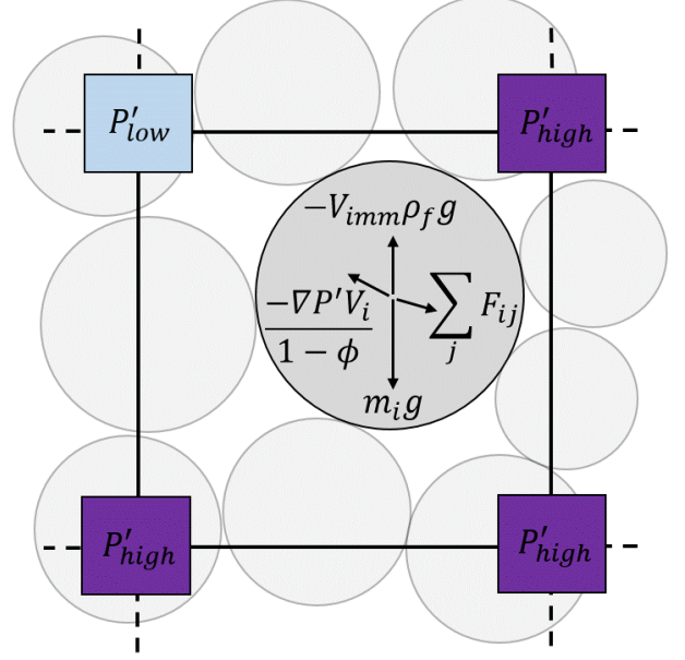
FIG. 1. Schematic representation of the forces in the model. Dynamic pore pressure gradients exert forces on each grain ( -(\nabla P' V_i)/(1 - \phi) ). These forces are inferred based on an interpolation scheme that interpolates the pressure gradients from grid nodes to the individual grains. As stated in Eq. (17), this force is added to gravity ( m_i \mathbf{g} ), buoyancy ( -V_{\text{imm},i} \rho_f \mathbf{g} ) and the sum of contact forces ( \sum_j \mathbf{F}_{ij} ).
