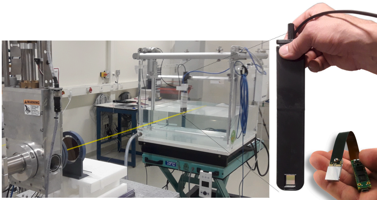
Fig. 14. Left: detector module for UHPDR beams based on MiniPIX TPX3 Flex in a water phantom in an ultra-high dose rate proton beam in the experimental room at OncoRay Dresden. Yellow line indicates the proton beam axis. Right: detection module. Bottom right: Original “MiniPIX-TPX3-Flex” detector.
