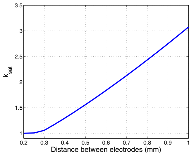
Fig. 11. Simulated ion recombination correction factor for a plane parallel air ionization chamber operated at 300 V as a function of the distance between electrodes for a pulse of 5 Gy with a 1 \mu s duration.
