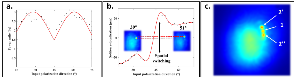
Fig. 2. a. Rogue event power ratio (compared to the whole beam) versus input polarization orientation at 0.66 \text{ GW/cm}^2 and \Delta k = 0 , b. Rogue event position evolution, for a variable input polarization orientation ( 0.66 \text{ GW/cm}^2 and \Delta k = 0 ), c. Multiple rogue event generation ( 0.66 \text{ GW/cm}^2 and \Delta k = 0 ).
