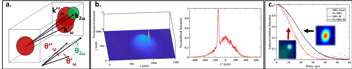
Fig. 1. a. Experimental setup, b. Extreme event at 0.3 \text{ GW/cm}^2 and \Delta k = 0 , ( left ) 3D view, ( right ) transverse beam profile, c. Autocorrelation profile of the crystal output beam with and without spatial trapping.
