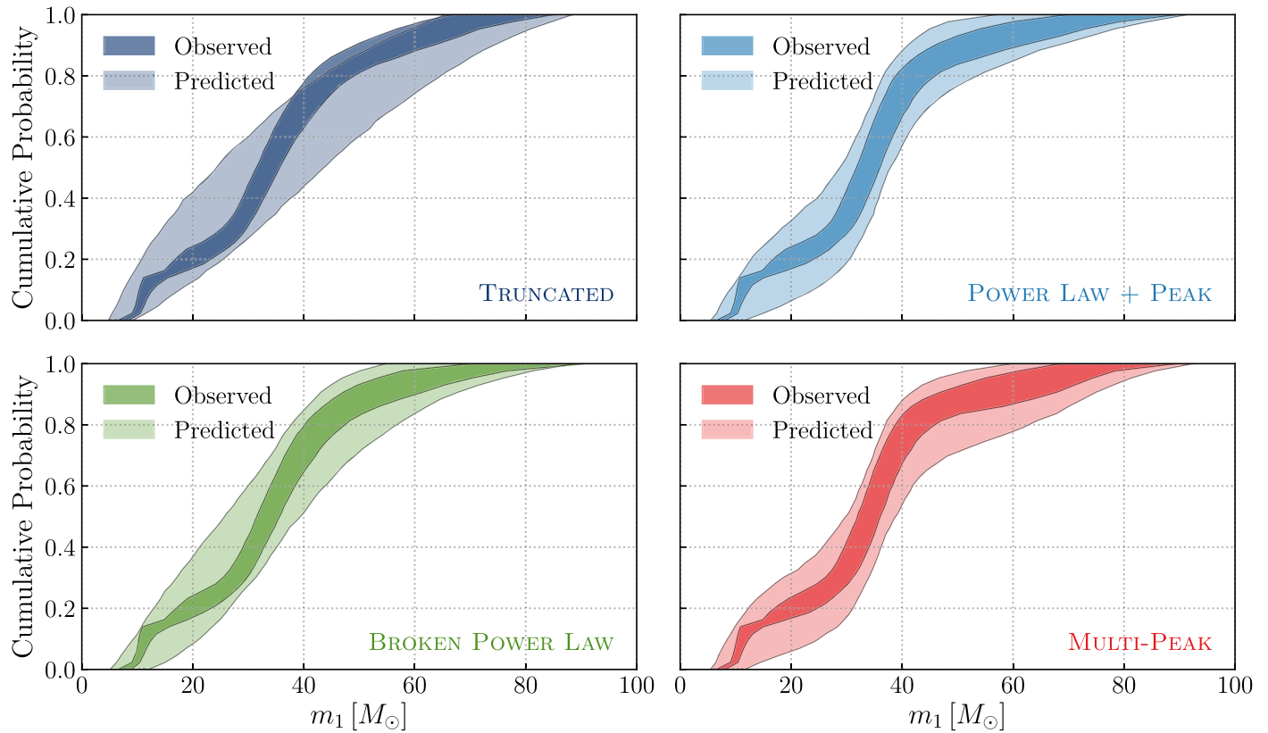
Figure 19. Posterior predictive check: the cumulative density function of the observed primary mass distribution for the TRUNCATED, POWER LAW + PEAK, BROKEN POWER-LAW, and MULTIPEAK models. The observed event distribution is shown with darker colors. The thickness of the bands indicates the 90% credibility range. The POWER LAW + PEAK, BROKEN POWER-LAW, and MULTIPEAK models are a better fit than the TRUNCATED MODEL; the dark band overlaps entirely with the light band. This is due to the POWER LAW + PEAK, BROKEN POWER-LAW, and MULTIPEAK models having more flexibility to fit the relative excess of binaries in the 30–40 M_\odot region compared to the \gtrsim 40 M_\odot region. This analysis excludes GW190814.
