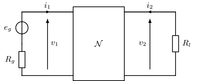
Fig. 1. Electronic filter \mathcal{N}
