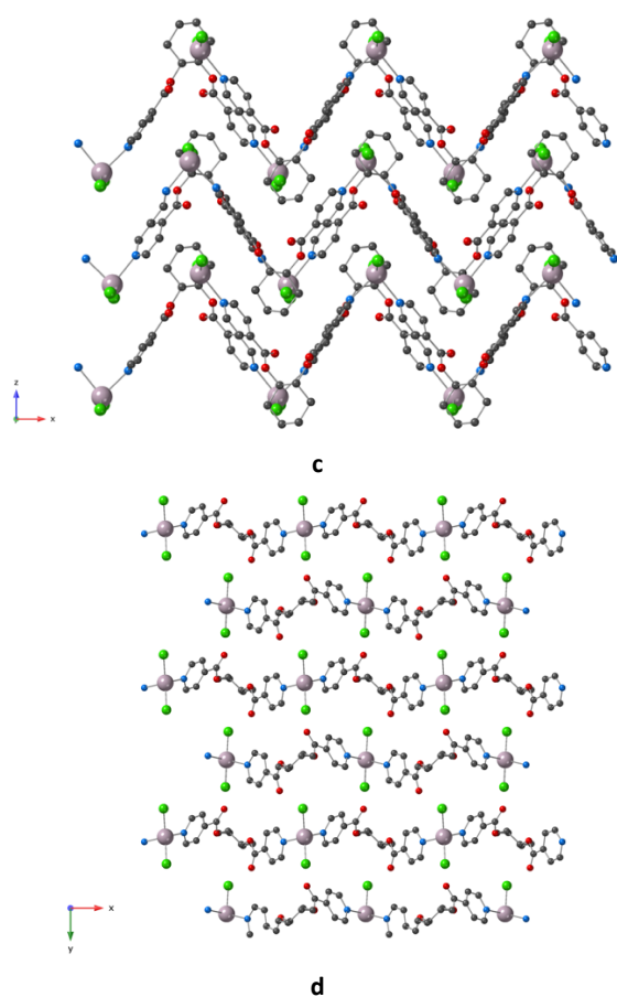
Figure 3. A portion of the 1D coordination networks 1a -HgCl 2 (or 1b -HgCl 2 ) along the a (picture a) and b (picture b) axes and corresponding packing obtained upon combining HgCl 2 with 1a (or 1b ) (pictures c and d, in the xOz and xOy planes respectively). H atoms are omitted for clarity of the representation.
