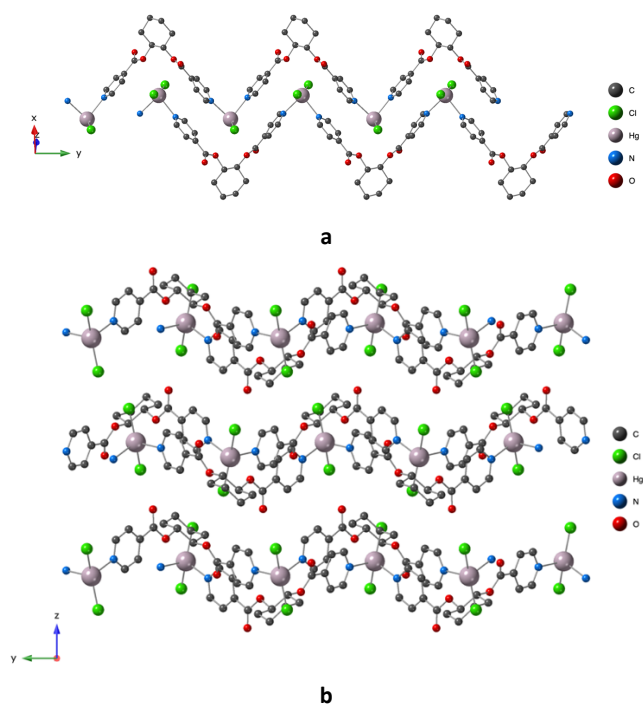
Figure 5. A portion of the chiral 1D coordination network 1a 0.5 1b 0.5 -HgCl 2 (a) and corresponding packing (b) obtained upon combining HgCl 2 with 1a+1b in racemic conditions. H atoms are omitted for clarity of the representation.
