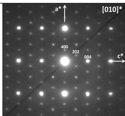
Figure 1. [010] selected area electron diffraction pattern of \alpha\text{-Rb}_3\text{AlF}_6 . Indexed in the a = 37.27 \text{ \AA} , b = 12.45 \text{ \AA} and c = 17.68 \text{ \AA} cell with a Fddd space group.
