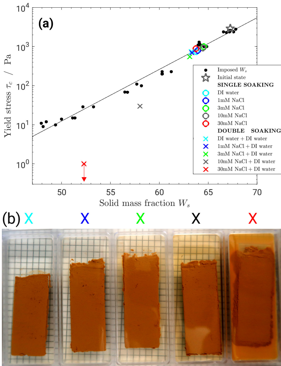
Fig. 5. Effect of NaCl concentration in the first soaking bath (0, 1, 3, 10 and 30 mmol/L). a) Yield stress as a function of the solid mass fraction after a single soaking (circles) or double soaking (crosses). The colors refer to the NaCl concentration during the first or single soaking, see the legend (the arrow below the red cross means that only a higher bound of the yield stress could be determined). b) Sediment samples at the end of double soaking (NaCl concentration during the first soaking increasing from left to right, the color of crosses at the top of the picture corresponds to the legend in Figure 5a). Soaking time: 24 hours in all cases. Sediment batch #2.
