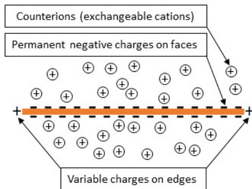
Fig. 2. Schematic view of a smectite particle.
