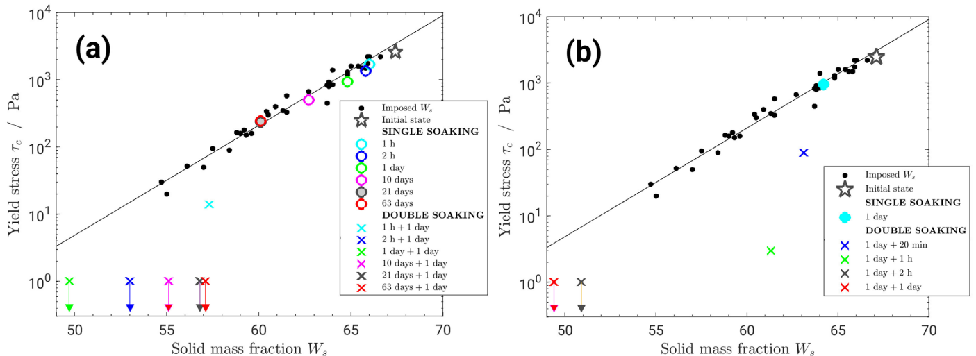
Fig. 6. Yield stress as a function of the solid mass fraction for different soaking times. a) First or single soaking in NaCl solution for various durations and second soaking in DI water for 24 hours. b) First or single soaking in the NaCl solution for 24 hours and second soaking in DI water for variable durations. The concentration of all NaCl solutions was 27 mmol/L. Sediment batch #1.
