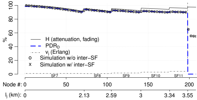
Figure 11: Large cell radius, density of 5 nodes per \text{km}^2 , SF boundaries for target PDR_D of 90%.
