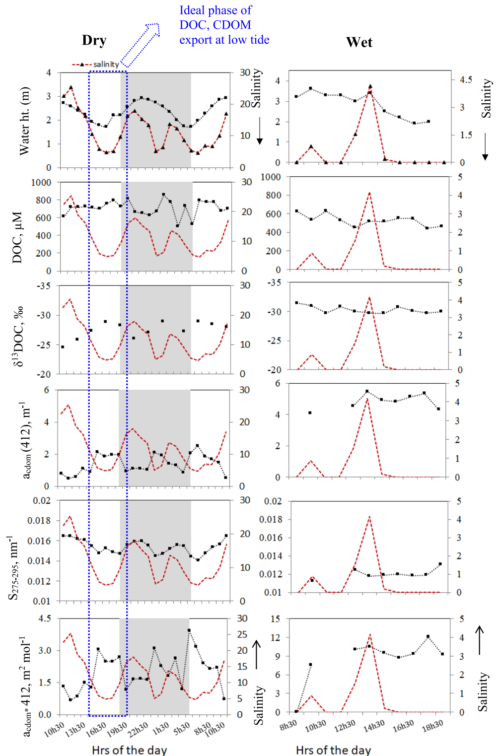
Figure 4. Tidal variations of surface water DOC ( \mu\text{M} ), \delta^{13}\text{C-DOC} (‰), and CDOM parameters like the absorption coefficient at 412 nm ( a_{\text{cdom}}(412) , \text{m}^{-1} ), slope at 275–295 nm ( S_{275-295} , \text{nm}^{-1} ) and CDOM normalized to DOC ( a_{\text{cdom}}*412 , \text{m}^2 \text{mol}^{-1} ) during the 24- and 12-hr surveys carried out in the dry and wet seasons of 2015, respectively. Tidal height (m) and salinity (red dashed line) are also represented on the figure. Vertical gray band representing the dark phase of the sampling period (18h30 to 5h30), and the blue box area describing the ebb tide period when mangrove-derived DOC and CDOM leaching was maximum as evidenced by stable isotope and optical indexes (refers to section. 4.3.1).
