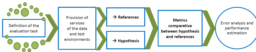
Figure 5: Automatic detection evaluation process
