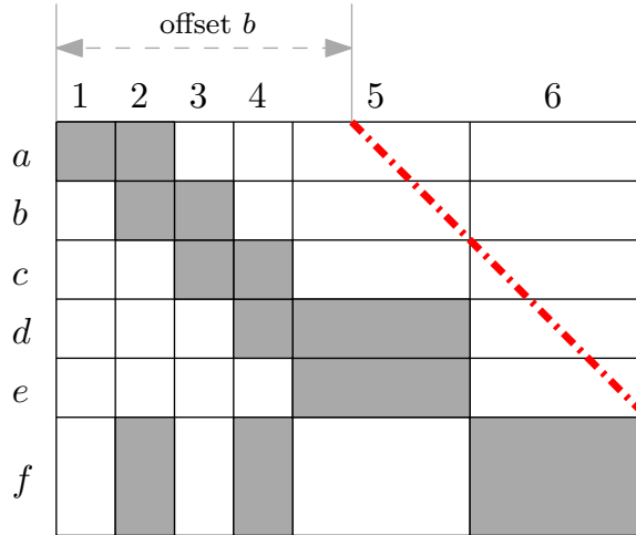
Fig. 5: Example of binary matrix visualization problem. Each row (resp. column) has its own height (resp. width).
