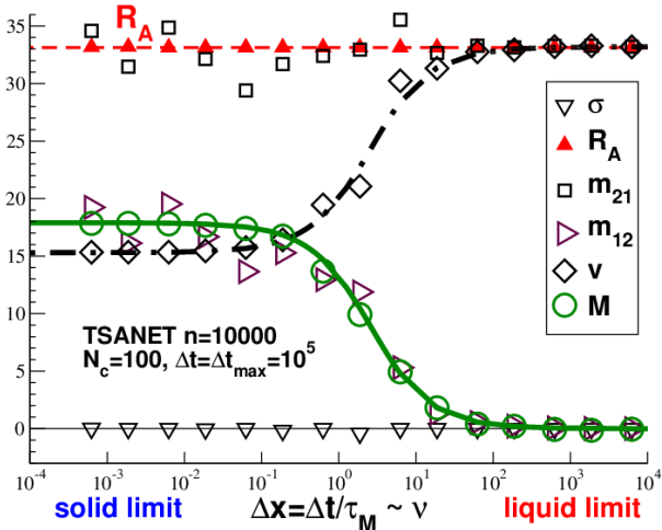
Fig. 6. Various properties obtained for the TSANET model vs. the reduced sampling time \Delta x = \Delta t/\tau_M for \Delta t = 10^5 : mean shear stress \sigma , affine shear modulus R_A , contributions m_{21} and m_{12} to the shear-stress fluctuation v = m_{21} - m_{12} and stress-fluctuation formula M = R_A - v for the shear modulus. The prediction for a Maxwell model is indicated by the bold solid line for M and by the dashed-dotted line for v . Note that R_A \approx m_{21} and M \approx m_{12} for all \Delta x .
