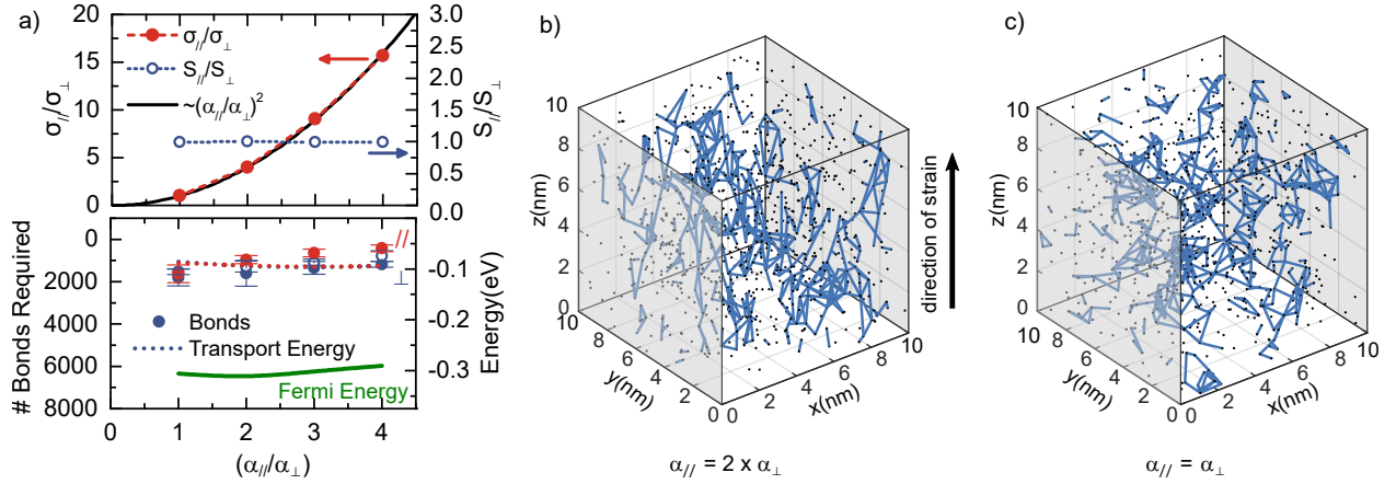
Figure 2: Hopping on a random lattice at a relative carrier concentration of c = 0.01 . a) Anisotropy in electrical conductivity \sigma_{//}/\sigma_{\perp} (filled red circles) and Seebeck coefficient S_{//}/S_{\perp} (open blue circles) (upper panel) and minimum number of bonds required until a path in the respective direction is reached (symbols) (lower panel) as a function of the anisotropy ratio. The dotted lines in the lower panel present the transport energy E_{tr} for the parallel (red) and perpendicular (blue) direction, respectively. The green line represents the Fermi energy E_F . b, c) Critical percolation cluster (blue lines) for hopping on a random lattice with \alpha = 0.4 \cdot [112] nm (b) and \alpha = 0.4 \cdot [111] nm (c). Black dots represent available sites, gray surfaces indicate the yz -planes.
