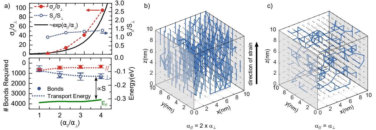
Figure 3: Hopping on a regular lattice at a relative carrier concentration of c = 0.01 . a) Anisotropy in electrical conductivity \sigma_{//}/\sigma_{\perp} (filled red circles) and Seebeck coefficient S_{//}/S_{\perp} (open blue circles) (upper panel) and minimum number of bonds required until a path in the respective direction is reached (symbols) (lower panel) as a function of the anisotropy ratio. The dotted lines in the lower panel present the transport energy E_{tr} for the parallel (red) and perpendicular (blue) direction, respectively. The green line represents the Fermi energy E_F . b, c) Critical percolation cluster (blue lines) for hopping on a regular lattice with \alpha = 0.4 \cdot [112] nm (b) and \alpha = 0.4 \cdot [111] nm (c). Black dots represent available sites, gray surfaces indicate the yz -planes.
