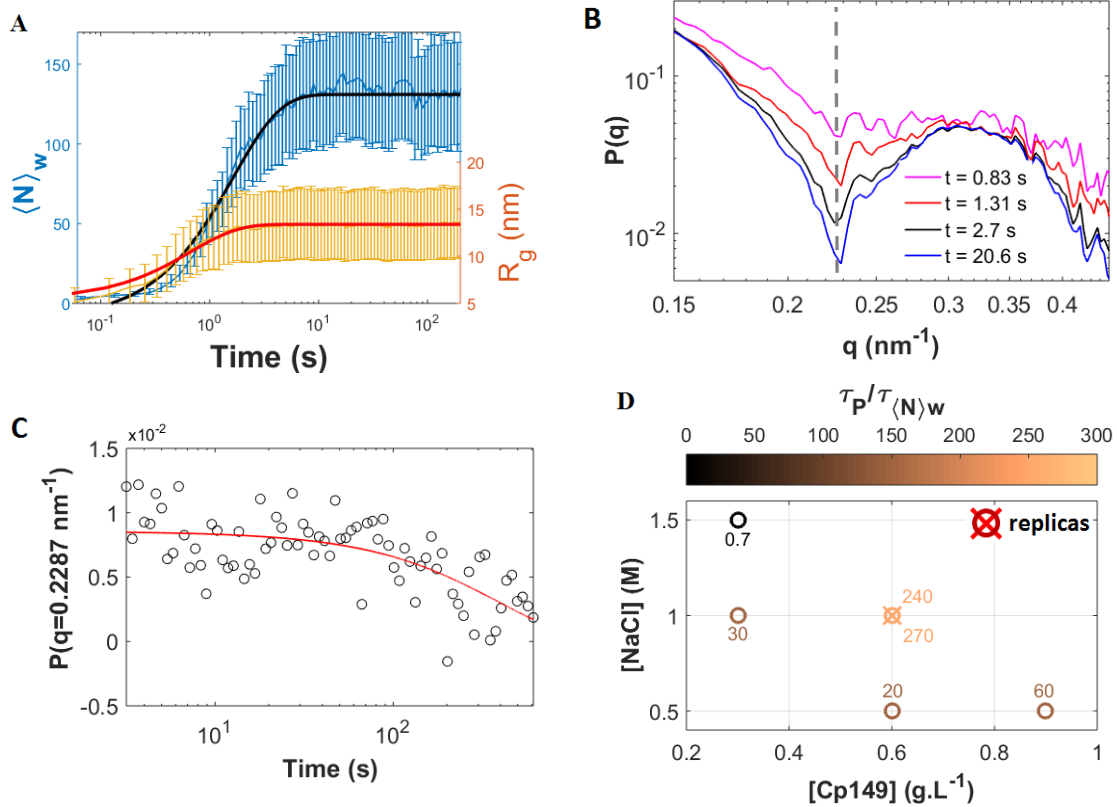
Figure 3: Assembly phases. (A) Evolution of \langle N \rangle_w (blue) and R_g (orange) as a function of time. The black and red curves show fits with a single exponential decay function. (B) Form factors P(q) at different time points. The gray dashed line indicates q = 0.2287 nm -1 . (C) Values of the form factors at q = 0.2287 nm -1 versus time. The red line is a single exponential decay fit yielding an estimate for the structural relaxation time \tau_P . (D) Summary graph of the ratios of the extracted characteristic timescales: \tau_P/\tau_{\langle N \rangle_w} .
