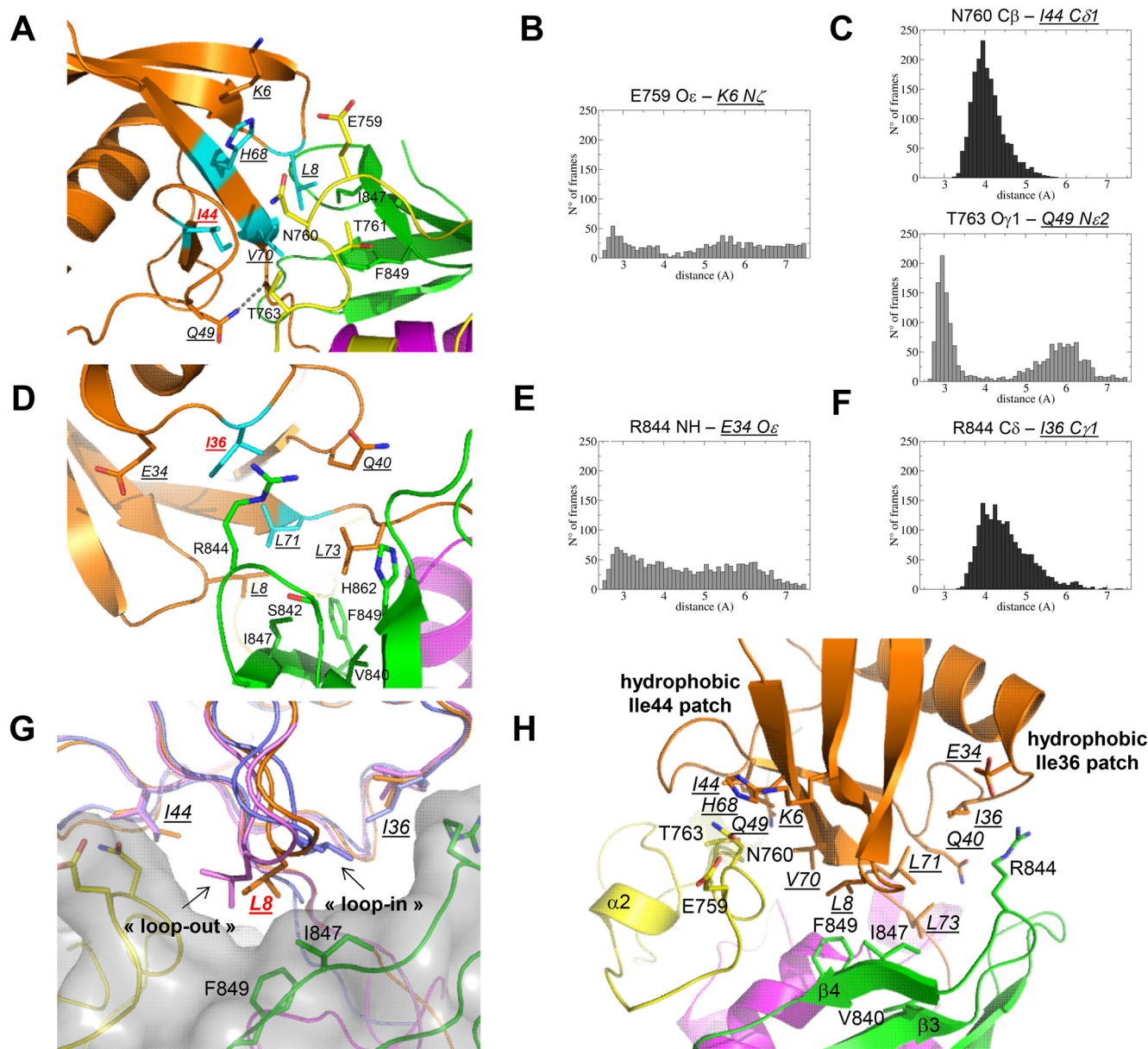
Figure 2. Interactions between TYMV PRO/DUB and Ub. A, close-up view of the Ub Ile 44 patch. Both proteins are shown in cartoon, and residues involved in the interaction are shown in stick. Proteins are colored as in Fig. 1, with oxygen and nitrogen atoms in red and blue, respectively. The hydrogen bond between Gln 49 from Ub and Thr 763 from TYMV PRO/DUB is shown as a dotted line. B and C, analysis of interactions around the Ub Ile 44 patch by molecular dynamics simulations. The distances between three pairs of residues were measured during 90 ns of production time in two simulations, and their frequency was plotted. Gray, hydrogen bonds and electrostatic interactions; black, hydrophobic contact. D, close-up view of the Ub Ile 36 patch. Proteins and residues are represented and colored as in A. E and F, analysis of interactions around the Ub Ile 36 patch by molecular dynamics simulations. The distances between two pairs of residues were measured during 90 ns of production time in two simulations, and their frequency was plotted, as in B and C. G, close-up view around Leu 8 of Ub. Both proteins are displayed in cartoon loop with some side chains shown in stick. The cavity of TYMV PRO/DUB that fits Ub is highlighted by the gray molecular surface of the enzyme. Three crystal structures of Ub were superimposed to compare the position of the loop encompassing Leu 8 : purple, loop-out conformation (PDB code 1UBQ (73)); orange, intermediate conformation (this work); blue, loop-in conformation (PDB code 2G45 (84)). H, overall view of the two polar loops of TYMV PRO/DUB that bind the two hydrophobic patches of Ub.
