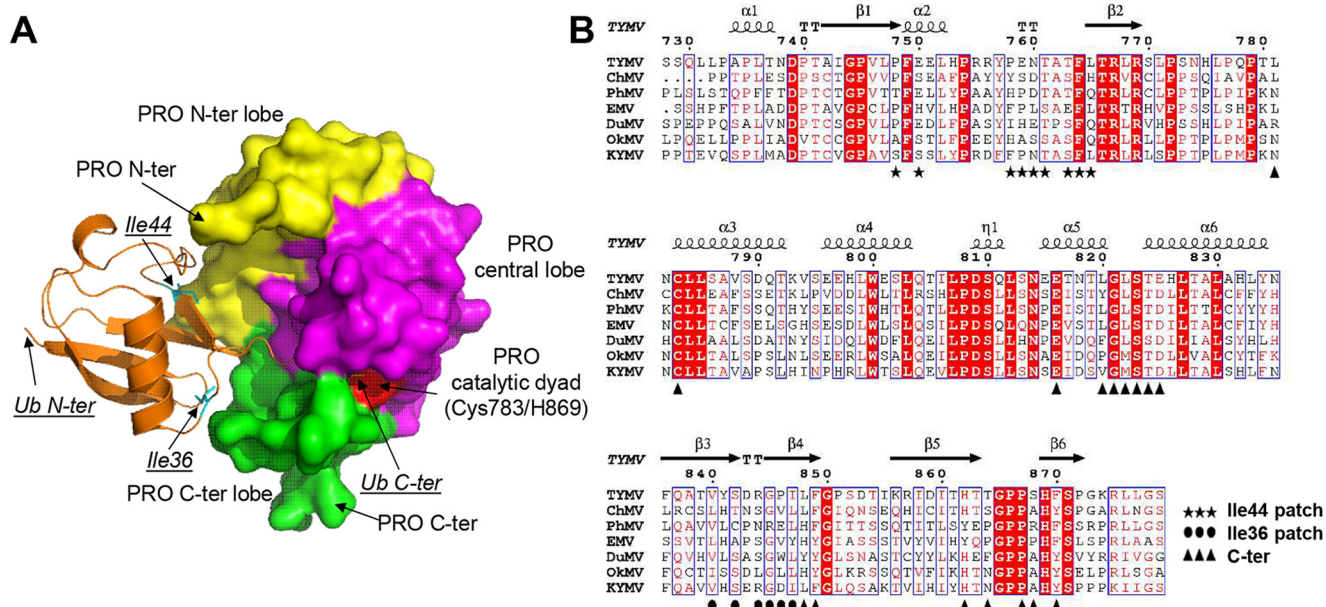
Figure 1. Overall structure of the covalent TYMV PRO/DUB–Ub complex. A, crystal structure of the covalent TYMV PRO/DUB–Ub complex. TYMV PRO/DUB is represented as molecular surface, with the N-terminal (N-ter) lobe in yellow, the central lobe in magenta, and the C-terminal (C-ter) lobe in green. The enzyme's catalytic dyad, composed of Cys 783 and His 869 , is indicated in red. HA–Ub–VME is shown in ribbon diagram and colored in orange. Residues Ile 36 and Ile 44 are displayed in ball-and-stick format and colored in cyan. Ubiquitin residues are labeled in italics and underlined . B, sequence alignment of polyprotein processing endopeptidases belonging to the Tymoviridae family. The sequence of TYMV PRO/DUB was aligned with enzymes encoded by Chayote mosaic virus (ChMV), Physalis mottle virus (PhMV), Eggplant mosaic virus (EMV), Dulcamara mottle virus (DuMV), Okra mosaic virus (OkMV), and Kennedy yellow mosaic virus (KYMV) as in the work of Lombardi et al. (34). Alignment was performed by CLUSTALW (82), edited, and displayed with ESPript3 (83). White characters in red boxes indicate identity, and red characters in white boxes indicate homologous residues. Secondary structures of TYMV PRO/DUB (PDB code 4A5U (34)) are indicated on top. Black stars indicate the residues of enzyme interacting with Ub Ile 44 hydrophobic patch, black circles indicate the residues interacting with Ub Ile 36 hydrophobic patch, and black triangles indicate the residues interacting with the C-ter extremity of Ub.
