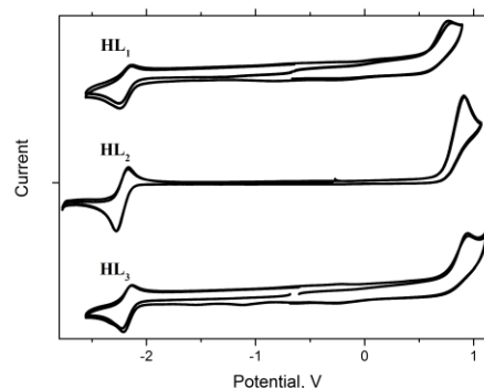
Figure 7. Cyclic voltammogram recorded for HL 1 , HL 2 and HL 3 in N 2 -purged DMF containing 0.1M TBAPF 6 vs Fc + /Fc at a glassy carbon working electrode.
