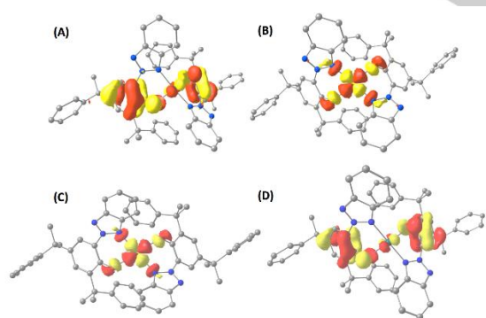
Figure 6. DFT-computed HOMO (A) and LUMO (B) for the neutral PdL 3 complex, SOMO for the mono-reduced PdL 3 (C) and SOMO for the one-electron oxidized PdL 3 (D). Hydrogen atoms were omitted for clarity.
