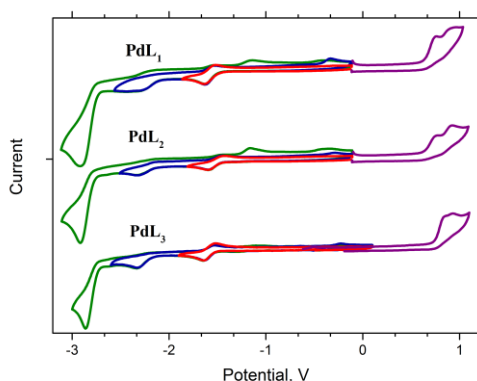
Figure 8. Cyclic voltammograms recorded for PdL 1 , PdL 2 and PdL 3 in N 2 -purged DMF containing 0.1M TBAPF 6 vs Fc + /Fc at a glassy carbon working electrode over different potential ranges both in the reduction mode (red, blue and green lines) and in oxidation mode (purple lines).
