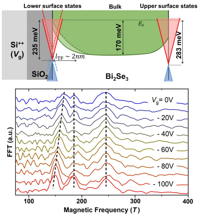
Figure 3. Band structure of a \text{Bi}_2\text{Se}_3 nanoribbon with the band bending measured close to the upper and lower surface states and the relative change of the band structure when a gate voltage is applied on the back-gate. The gate dependence of the Fourier transform of the Shubnikov–de Haas oscillations in the \text{Bi}_2\text{Se}_3 nanoribbon is shown below. Three different peaks can be clearly observed. Based on their gate dependence and on considerations of the effective mass, they could be assigned to the different charge carriers (upper and lower surface states as well as bulk states). Adapted with permission. [14] Copyright 2016, American Chemical Society.
