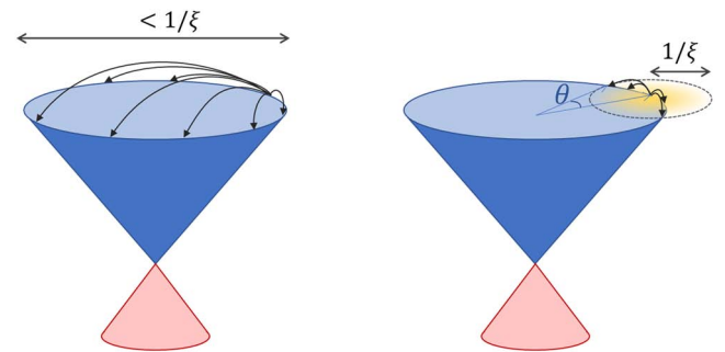
Figure 6. Illustration of an isotropic scattering (left) and anisotropic scattering (right). In the isotropic scattering, all the states at the Fermi energy are equally accessible, whereas the available states are restricted in a small area (in yellow) close to the initial state with a small \theta angle for an anisotropic scattering. The cutoff that determine the available state is given by \approx 1/\xi .
