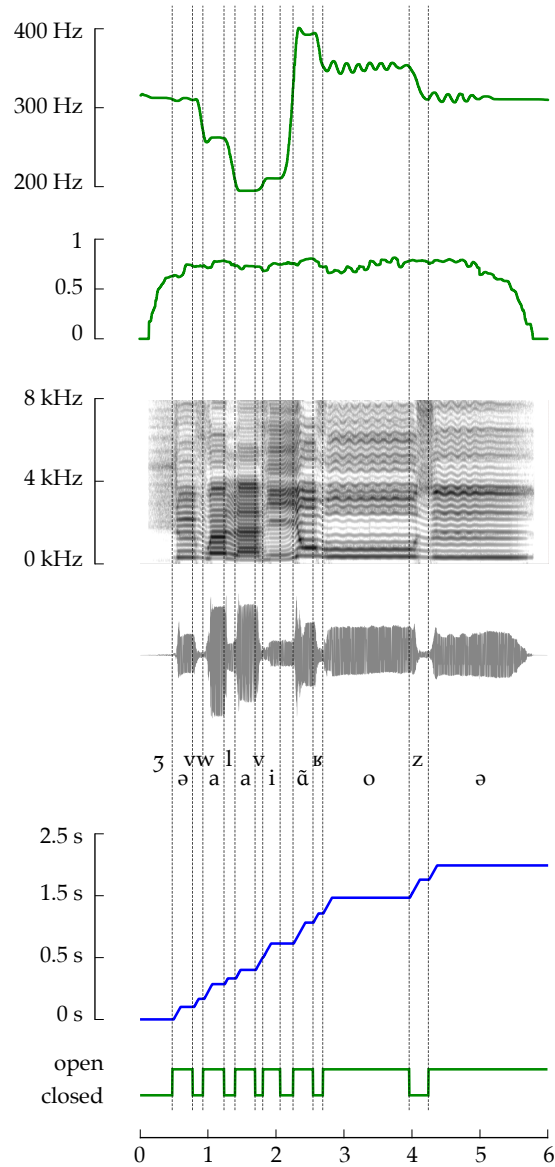
Figure 3: Performance using Voks in the syllabic control mode. French sentence "Je vois la vie en rose" (/ʒəvwalaviãbozə/, duration 2.5 s). Synthesis duration: 6s. Input control data in green, internal data in blue, output audio in greyscale. From top to bottom: pitch, normalized vocal effort, spectrogram, oscillogram, phonemic labels, internal time index \tau (blue), binary rhythm control (green). Times at which the rhythm controller is pressed or released are marked with a vertical dotted line.
