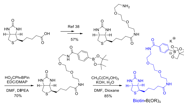
Scheme 3 Synthetic route of the biotin cyclic triolborate probe.
