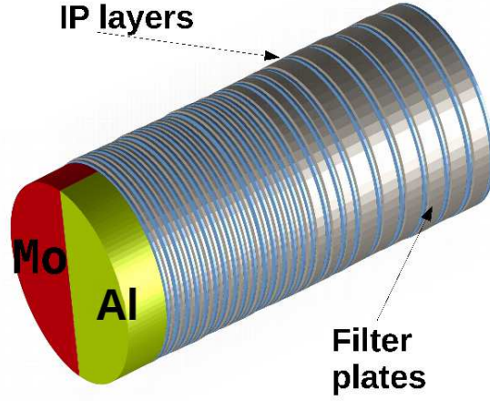
FIG. 1. Schematic view of the Bremsstrahlung cannon stack with split front filter.
