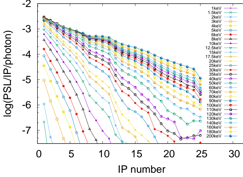
FIG. 5. Calculated response curves (PhotoStimulated Luminescence (PSL)/Image Plate (IP)/photon) of the 25 Image Plate layers in the Bremsstrahlung cannon stack to a single-temperature Maxwell-Boltzmann photon distribution for temperatures in the range 1 – 200 keV for the Al filter channel.
