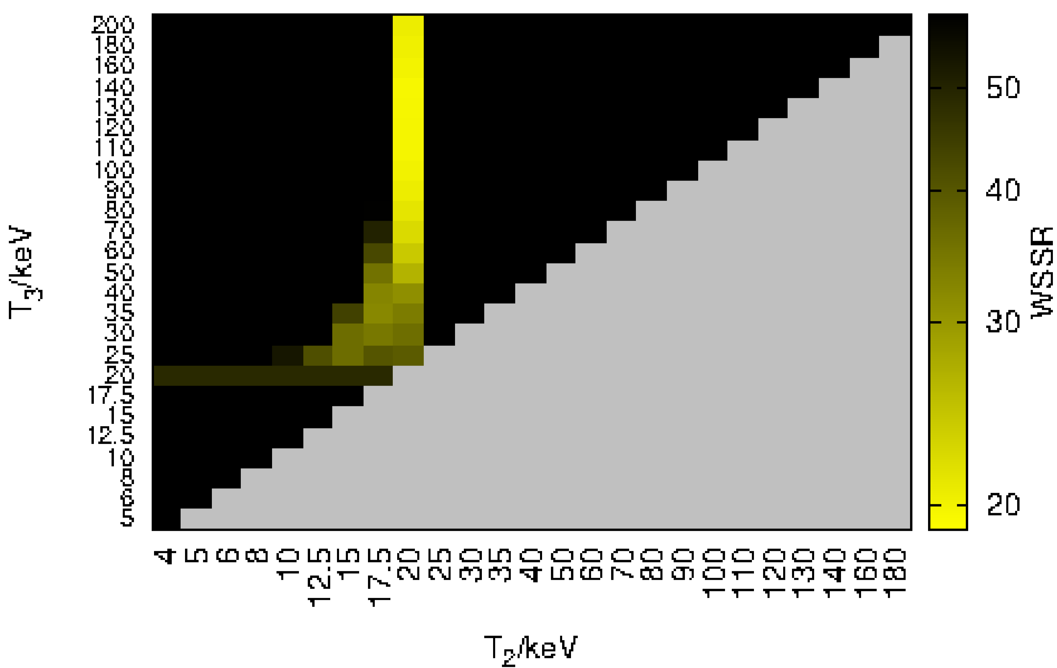
Shot1: Al channel ( T_1 = 3 keV)
