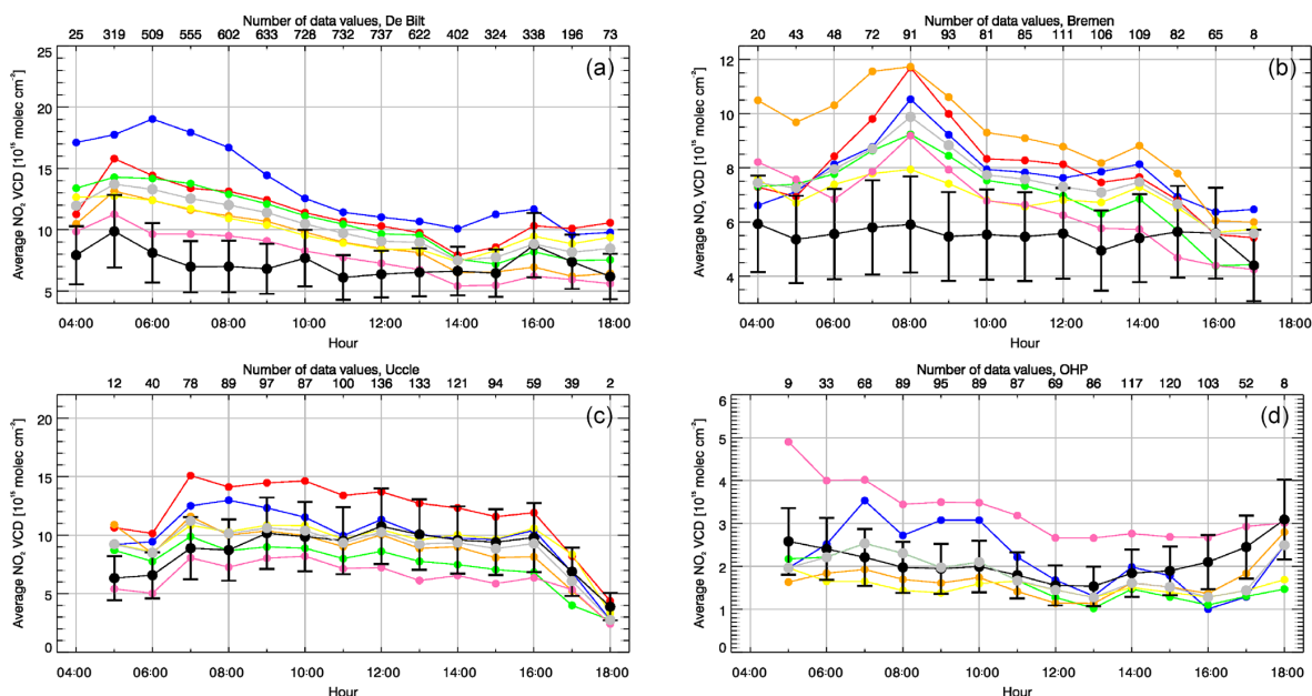
Figure 10. As in Fig. 8 but for diurnal cycles (averages over hourly bins) of tropospheric NO 2 VCDs ( 10^{15} molec cm -2 ) during weekends only.
