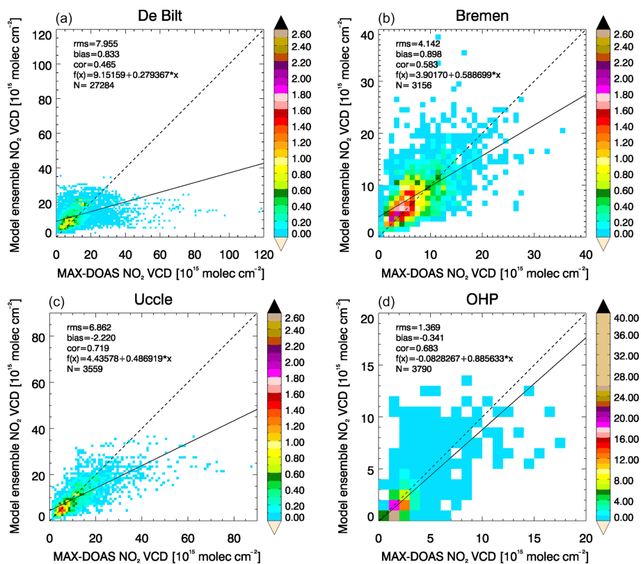
Figure 6. Scatter density plots of AVK-weighted tropospheric NO 2 VCDs (10 15 molec cm -2 ) from MAX-DOAS against model ensemble data for (a) De Bilt, (b) Bremen, (c) Uccle and (d) OHP. The data are shown for different bins with a size of 10 15 molec cm -2 and are colored according to the number of data points per bin (%). The dashed line is the reference line ( f(x) = x ). The solid line is the regression line (see top left of each plot for f(x) of this line). The root mean squared error (RMSE) (10 15 molec cm -2 ), bias (10 15 molec cm -2 ), Pearson correlation coefficient (cor, not squared) as well as the number of data points N are given in the top left of each plot.
