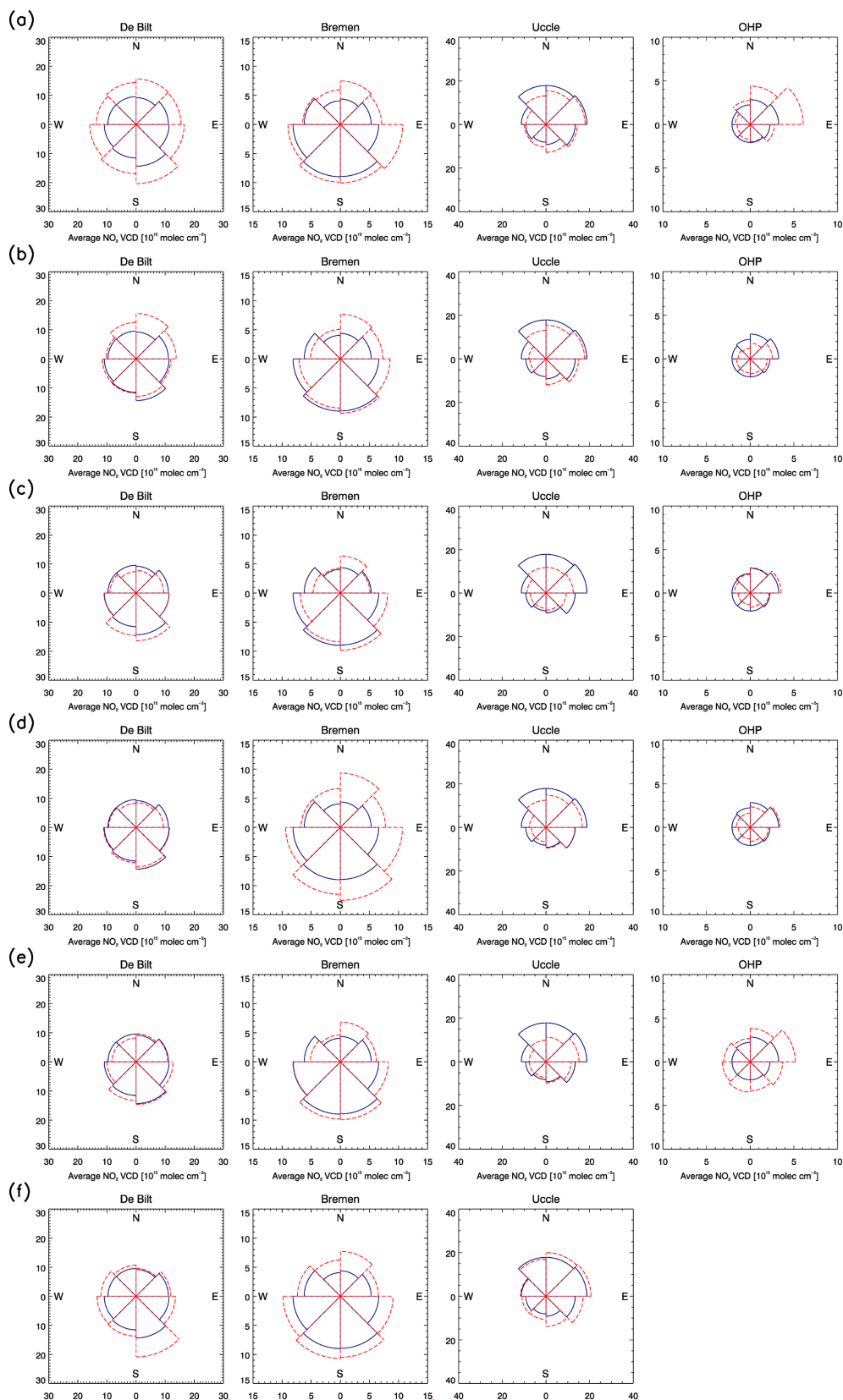
Figure A3. As in Fig. A2 but for average AVK-weighted tropospheric NO 2 VCDs ( 10^{15} \text{ molec cm}^{-2} ) in 45^\circ wide wind direction bins from (solid blue lines) MAX-DOAS and (dashed red lines) model data calculated. MOCAGE data are not available for the measurement time period at OHP.
