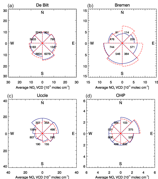
Figure 7. Average AVK-weighted tropospheric NO 2 VCDs ( 10^{15} molec cm -2 ) in 45° wide wind direction bins from (solid blue lines) MAX-DOAS and (dashed red lines) model ensemble data for (a) De Bilt, (b) Bremen, (c) Uccle and (d) OHP. Wind directions correspond to the direction towards the station and are taken from weather station measurements. The numbers close to the center of each plot refer to the number of data values used for calculating average values for each bin.
