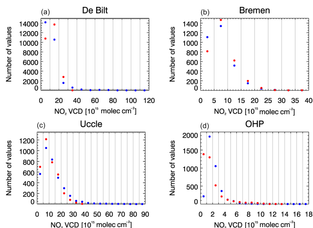
Figure 4. Frequency distributions of AVK-weighted tropospheric NO 2 VCDs ( 10^{15} molec cm -2 ) from (blue) MAX-DOAS and (red) model ensemble data for (a) De Bilt, (b) Bremen, (c) Uccle and (d) OHP. The distance between vertical gray lines on the x axis corresponds to the size of the bins used to calculate the number of values given on the y axis.
