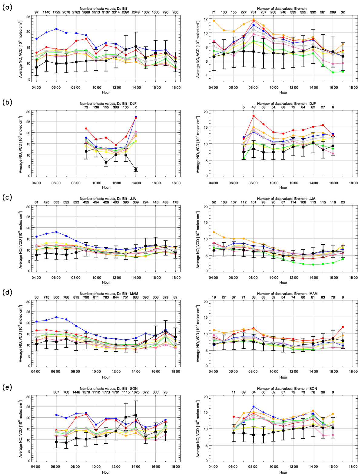
Figure A4. Diurnal cycles (averages over hourly bins) of AVK-weighted tropospheric NO 2 VCDs ( 10^{15} molec cm -2 ) from (black) MAX-DOAS, (gray) model ensemble median, (blue) LOTOS-EUROS, (yellow) CHIMERE, (green) EMEP, (orange) EMEP-MACCEVA, (pink) SILAM and (red) MOCAGE for (left) De Bilt and (right) Bremen. Model-based diurnal cycles were calculated from tropospheric NO 2 VCDs. Black error bars refer to the uncertainty associated with the MAX-DOAS retrievals (assumed to be 30% for all stations). Panel (a) shows cycles for the whole time series, (b) shows cycles for DJF, (c) MAM, (d) JJA and (e) SON months only. The number of data values used for calculating average values is shown in the top x axis of each plot.
