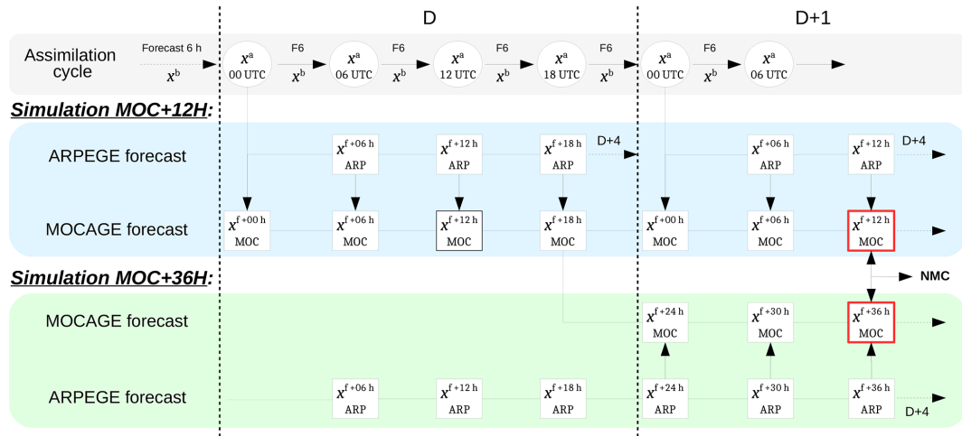
Figure 5. Schematic illustration of the NMC method using MOCAGE CTM, where x_{\text{MOC}}^{f+12\text{h}} is the forecast from simulation MOC+12H that is valid at time D . Similarly, x_{\text{MOC}}^{f+36\text{h}} is the forecast from simulation MOC+36H that is valid at time D + 1 .
